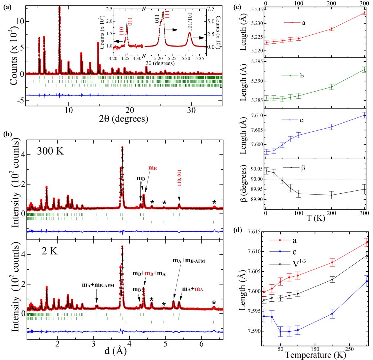
FIG. 4. Results for the nominal Ca_{0.5}Mn_{1.5}FeReO_6 ( x = 0.5 ) sample. Fits to (a) 300-K PSXRD and (b) 2- and 300-K PND profiles. The x = 0.5(T) phase is indicated with red labels, while the x = 0.5(M) phase is indicated by black labels. Designations m_A/m_B indicate reflections that have magnetic contributions from A- or B-site spin order and m_{B-AFM} refers to the antiferromagnetic component of Fe/Re spin order along the b axis due to frustration. Asterisks mark a small MnFe_3O_5 impurity. Thermal variations of PND lattice parameters for (c) x = 0.5(M) and (d) x = 0.5(T) phases.
