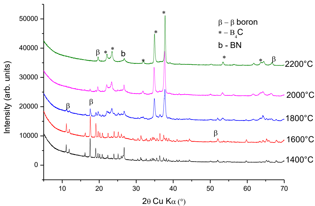
Figure 2: ex-situ x-ray diffraction pattern of quenched sample from a mixture of crystalline boron and amorphous carbon under 2 GPa in the Paris-Edinburgh cell for 2 hours at various temperatures.
