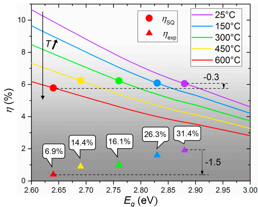
Figure 5. Analysis of the Efficiency of InGaN/GaN Multiple Quantum Well Solar Cells Tested under 1-Sun Illumination as a Function of Temperature
