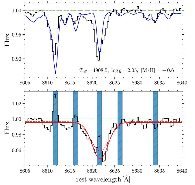
Fig. 3. Gaussian model for CIS of the star HD 149349 observed by the RAVE survey ( R = 7500 ). Upper panel: black and blue lines show the observed and synthetic spectra, respectively. The atmospheric parameters from RAVE-DR6 are also indicated. Lower panel: renormalized interstellar spectrum represented by the black line. The dashed and solid red lines represent the profiles from the first and second (finally selected) fits, respectively. The blue shades indicate the masked regions discussed in Sect. 2.6.2.
