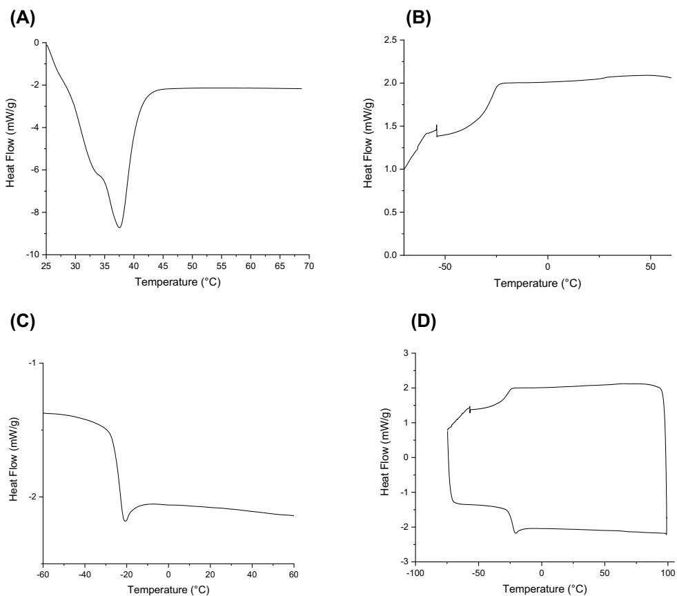
Figure S10. Thermal analysis of PTMC 30 -N 3 by differential scanning calorimetry (DSC) thermograms (10°C/min) (A) first heating (B) cooling (C) second heating (D) an entire cycle.
