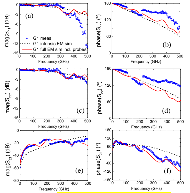
Fig. 11. S-parameters in magnitude (a),(c),(e) and phase (b),(d),(f) of the transistor short structures comparing the measurement (symbol) and the EM simulation (dashed line=intrinsic device simulation, straight line=complete device simulation including RF pads and probes + TRL calibration).
