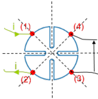
Figure 14 - Resistance measurement method using a cloverleaf sample
