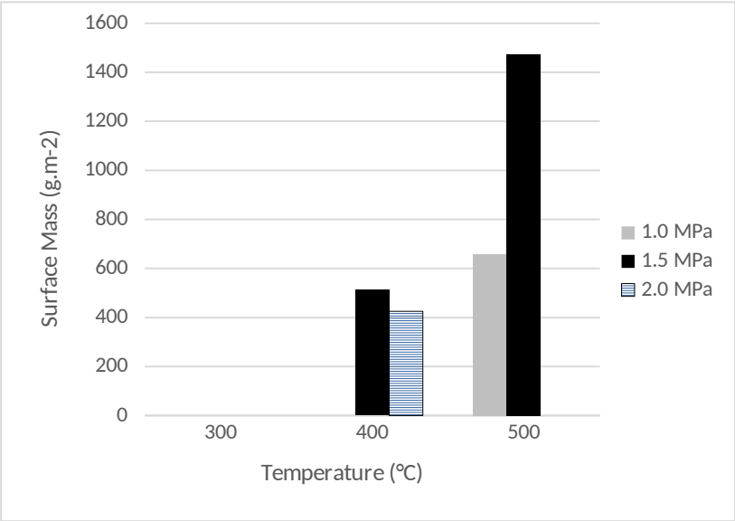
Figure 5 - Surface mass of the coatings containing irregular copper depending on gas temperature and pressure
