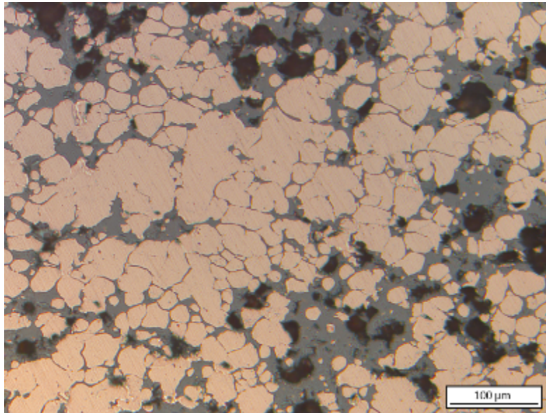
Figure 19 – Optical image (cross-section) of a heterogeneous coating made of non-oxidized copper particles
