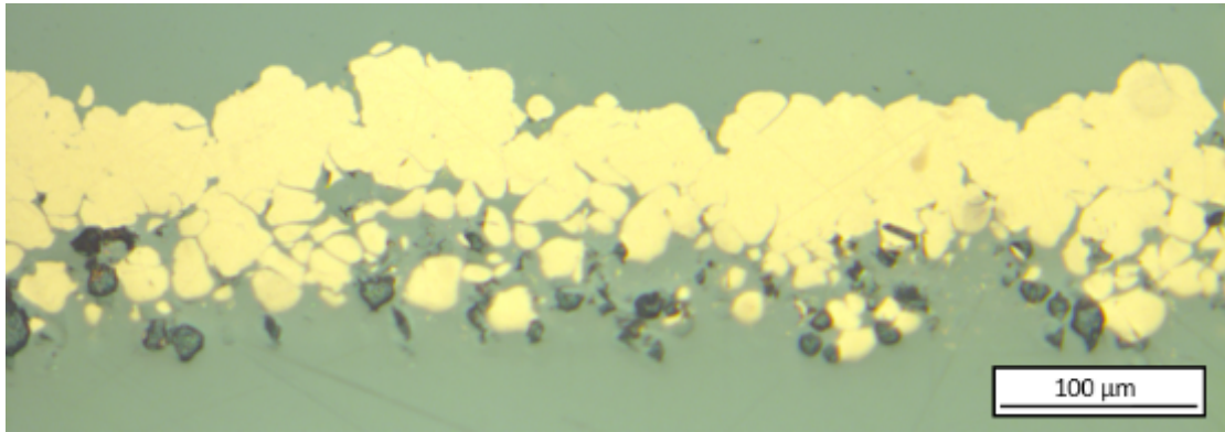
Figure 17 – Optical microscope image of a cross-section of cold-sprayed copper coating onto PEEK
