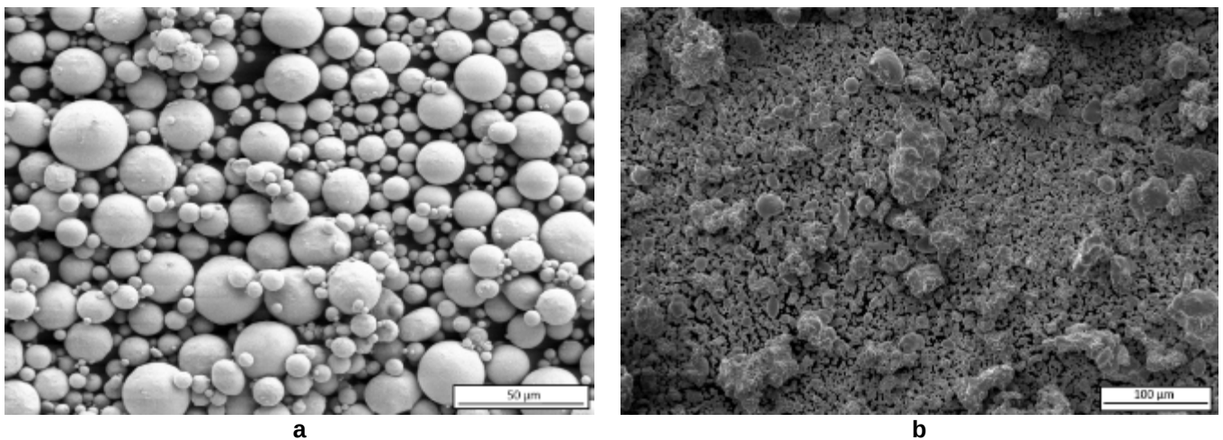
Figure 1 – SEM view of spherical (a) and irregular copper powders (b)
