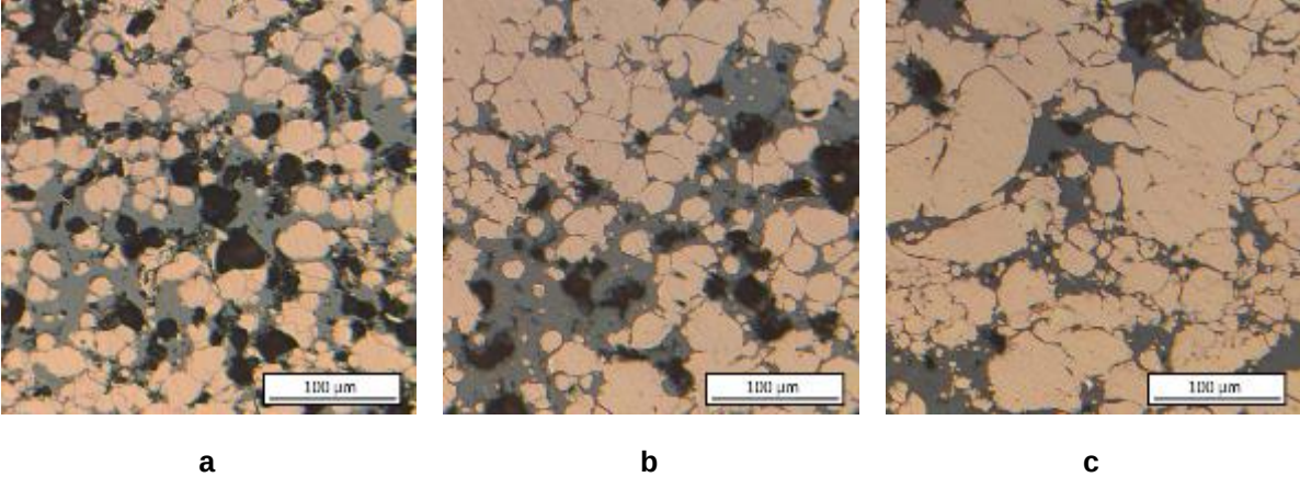
Figure 8 - Optical cross-section view of Cu-PEEK composite coatings with (a) spherical oxidized, (b) non-oxidized and (c) irregular copper
