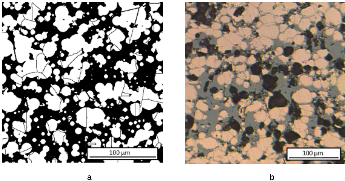
Figure 10 - Simulated (a) and experimental (b) images of a microstructure made of PEEK + oxidized copper
