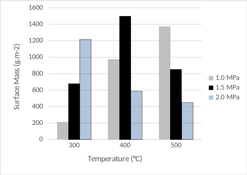
Figure 4 - Surface mass of the coatings containing oxidized spherical copper depending on gas temperature and pressure
