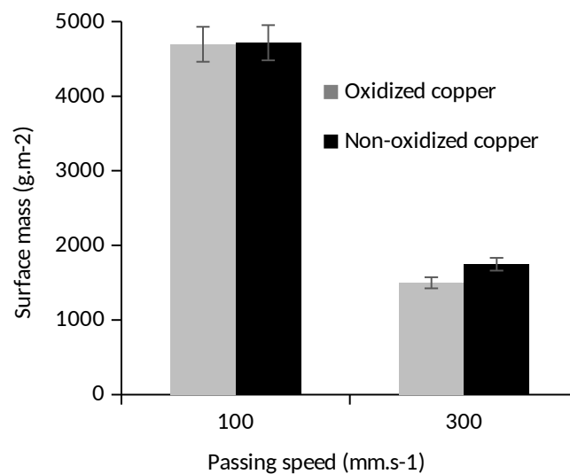
Figure 6 - Influence of cold spray parameters on the surface of coatings with oxidized spherical copper
