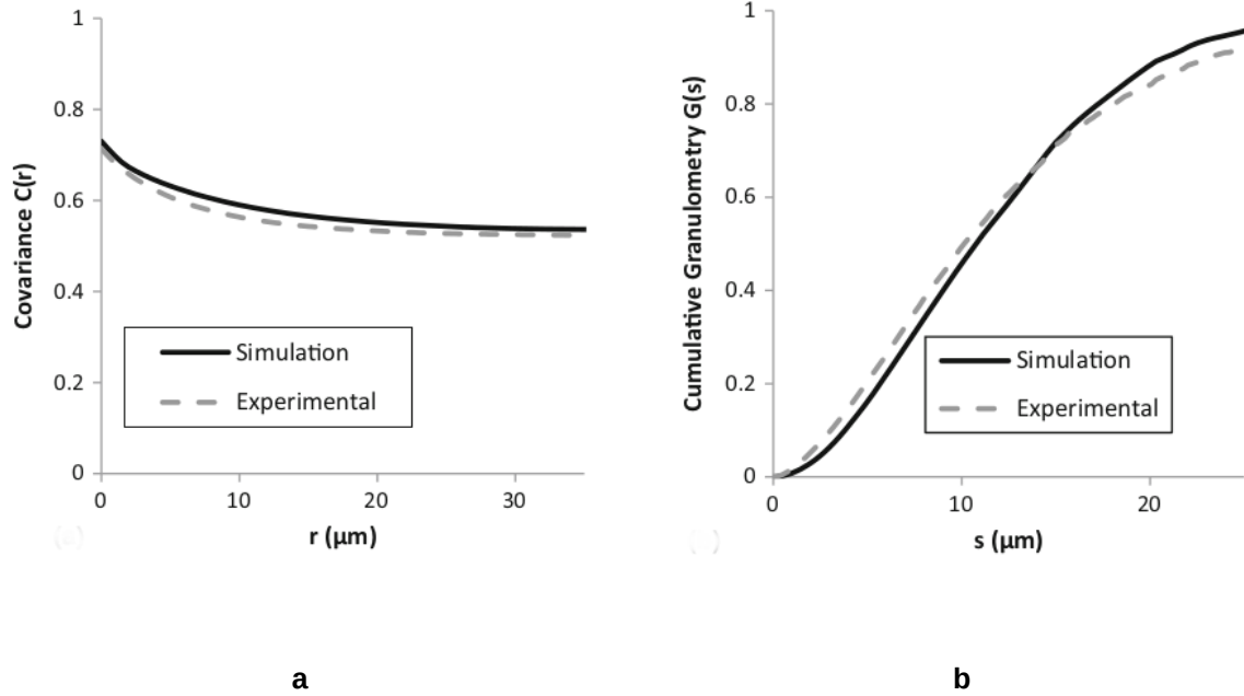
Figure 13 – Mean covariance and granulometry of experimental and simulated microstructures
