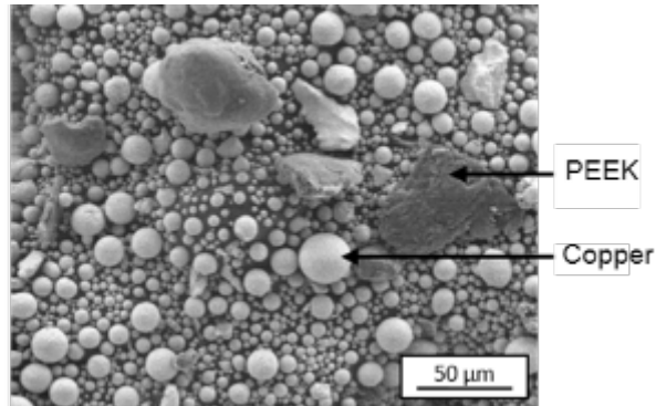
Figure 2 – SEM view of a spherical copper-PEEK powder blend
