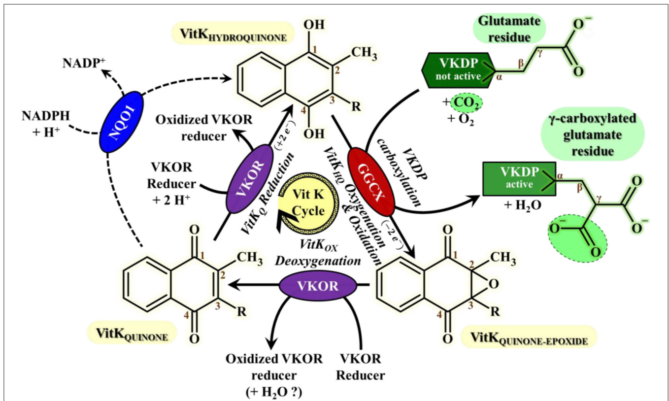
FIGURE 1 | Vitamin K cycle most important features for VKAs mode of action understanding This cycle consists in the recycling of vitamin K HydroQuinone (VitK HQ ) state, the sole active Vitamin K redox-state involved in the carboxylation mechanism of VKDPs catalyzed by the GGCX enzyme. The recycling of VitK HQ needs the deoxygenation of Vitamin K Quinone-Epoxyde state (VitK QX ) only catalyzed by VKOR enzymes, followed by bielelectronic reduction of Vitamin K Quinone state (VitK Q ) mainly catalyzed by VKOR enzymes and by an alternative enzyme which current consensus is NQO1 (68). Gamma-Carboxylation of glutamates residues from Vitamin K Dependent proteins (VKDP) catalyzed by GGCX is required for activation of VKDPs proteins, including essential clotting factors. The regeneration of the reduction power of VKOR is sustained by a “VKOR reducter” that is much likely, as far as we know, a protein partner probably from PDI-like enzymes family. VKOR stands for VKORC1 or VKORC1L1; GGCX, Gamma-Glutamyl Carboxylase; NQO1, NADPH:Quinone Oxidoreductase 1; VKDP, Vitamin K-Dependent Protein; VitK Q , Vitamin K Quinone form; VitK HQ , Vitamin K Hydroquinone form; VitK QX , Vitamin K quinone-epoxide form.
