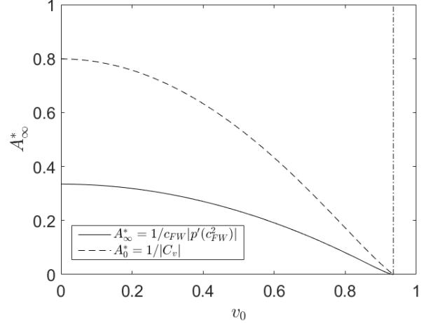
FIG. 10. Full line: FW normalized amplitude A_\infty^* = A(t/\lambda_z \gg 1)/\gamma_0 as a function of crack speed, v_0 . Dash line recalls the variations of A^*(t=0 = -1/C_v(v_0)) with v_0 [Fig. 3(a)]. Here, c_{FW}^0 , c_{FW} and v_0 are normalized by c_S . Poisson ratio is set to \nu = 0.35 , so that c_D = 2.082 and c_R = 0.935 . All speeds are expressed in c_S unit
