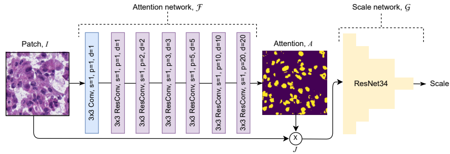
Fig. 1. A diagram of our approach. Each patch I is fed to the attention network \mathcal{F} generating an attention map A . The “attended” image J is then given to the scale classification network \mathcal{G} . Both networks are trained in an end-to-end fashion. s , p , and d for convolution blocks refer to stride, padding, and dilation.
