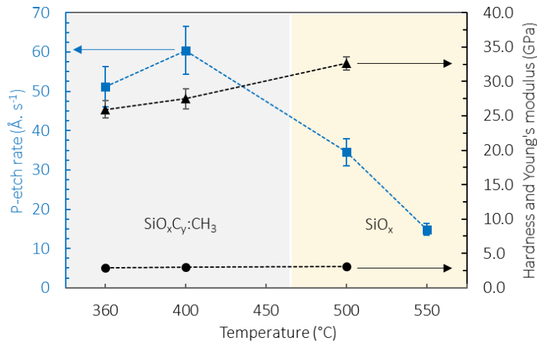
Fig. 9. Performance of HMDS-TEOS films in terms of corrosion resistance and mechanical properties. Evolution of Pliskin-test wet etching rates (squares), Young's modulus ( triangles ) and hardness values ( circles ) from nanoindentation analysis, plotted versus various SP temperatures. Grey and off-white regions signify \text{SiO}_x\text{C}_y:\text{CH}_3 and \text{SiO}_x material domains respectively.
