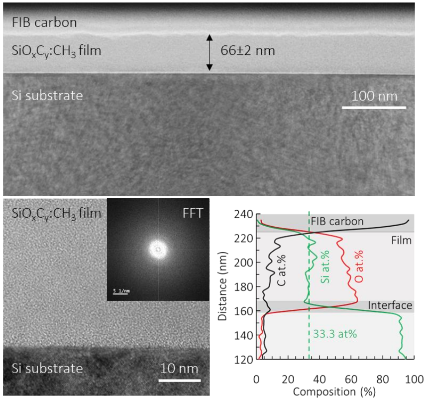
Figure 7. TEM analysis of a HMDS-TEOS SP360 film. Cross section (top), high-resolution cross section and Fast Fourier Transform (bottom left), and EDS elemental profile (bottom right).
