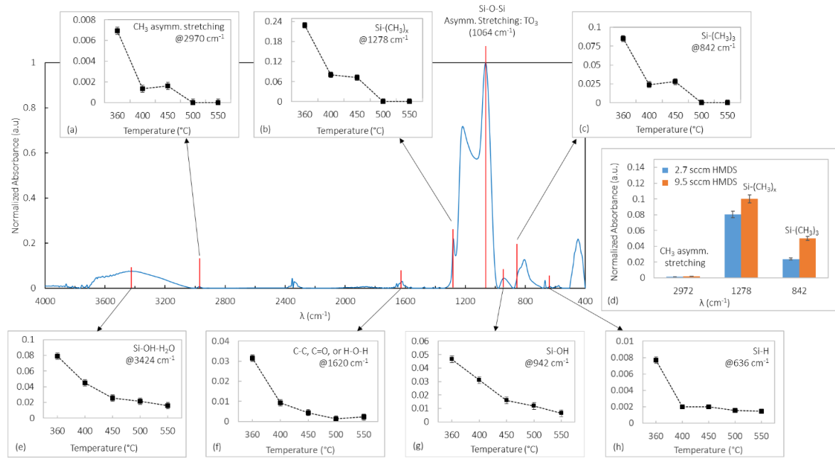
Figure 3. FTIR survey spectrum of a HMDS-TEOS film deposited at 360°C, analyzed for an incidence angle of 60°. Inset diagrams show the intensity’s evolution of the CH 3 asymmetric stretching (a), the CH 3 symmetric bending in Si-(CH 3 ) x (b) and rocking CH 3 vibration in Si-(CH 3 ) 3 (c) as a function of the SP temperatures. Inset histogram (d) shows these three absorptions for two different HMDS flow rates, at SP400. The remaining inset figures show the evolution of water-bonded silanol (e), water (f), free Si-OH (g) and Si-H (h) absorptions with the SP temperature.
