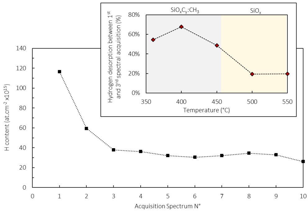
Figure 6. Hydrogen content of an SP400 HMDS-TEOS film as analyzed by 10 consecutive ERDA spectra acquisitions. Inset figure shows evolution of the percentage of hydrogen desorption between the first and third spectral acquisitions as a function of the SP temperature.
