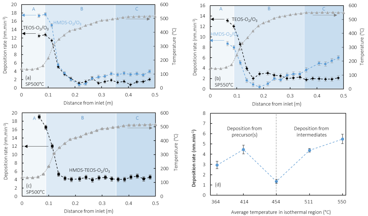
Figure 1. Typical thermal and deposition profiles for HMDS, TEOS, and HMDS-TEOS films. Deposition profiles from TEOS (black diamonds) and HMDS (blue squares) chemistries, at SP500 (a) and SP550 (b). Deposition profile from HMDS-TEOS dual-precursor chemistry at SP500 (c). Blue areas signify the low temperature region at the inlet (A), the gradient temperature region (B) and the isothermal region (C). Corresponding thermal profiles are shown by grey triangles in all three diagrams. (d) Average deposition rates for HMDS-TEOS films taken from the isothermal region (C) from runs performed at various SP temperatures.
