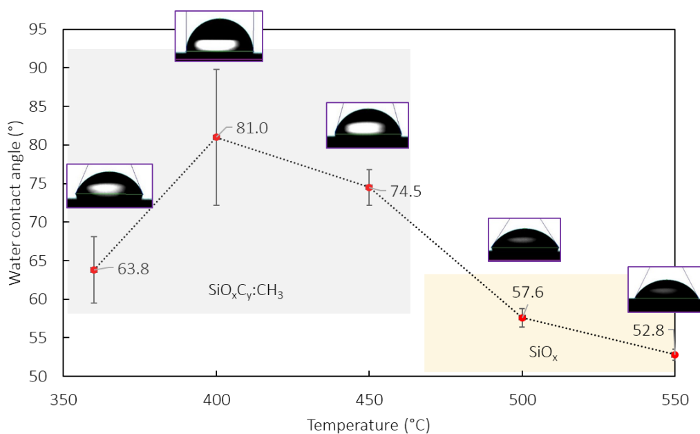
Figure 8. Water contact angles for HMDS-TEOS films and their evolutions as a function of the SP temperature. Grey and off-white regions signify \text{SiO}_x\text{C}_y:\text{CH}_3 and \text{SiO}_x material domains respectively.
