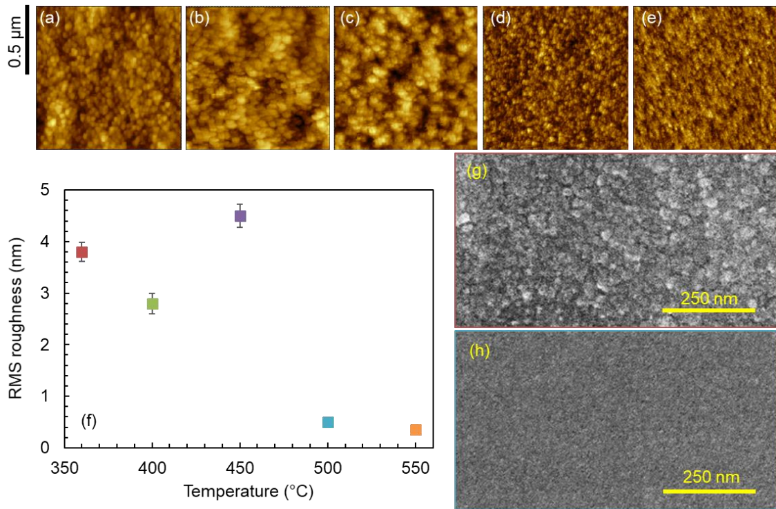
Figure 2. Surface topography and roughness of HMDS-TEOS films at various SP temperatures. AFM 1\mu\text{m}^2 surface topography at SP360 (a), SP400 (b), SP450 (c), SP500 (d) and SP550 (e). RMS roughness of HMDS-TEOS films for different temperatures measured by AFM (f). Inset images show SEM surface morphology for SP360 (g) and SP500 (h).
