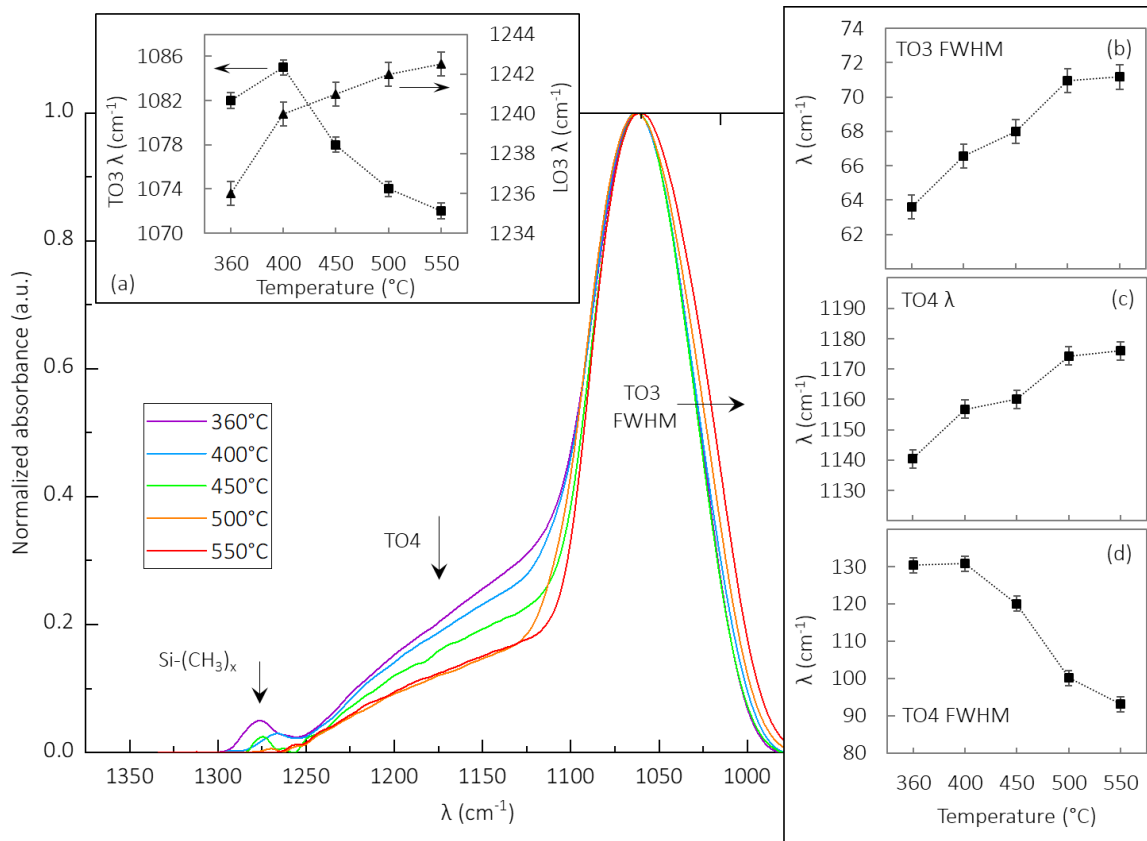
Figure 4. Evolution of the FT-IR spectrum of HMDS-TEOS films deposited at various SP temperatures, analyzed for an incidence angle of 0^\circ . Inset diagram (a) shows the evolution of the TO3 and LO3 components, as observed for an incidence angle of 60^\circ . Right hand-side inset diagrams show 0^\circ angle evolution of the TO3 full width half maximum (b), the TO4 position (c), and the TO4 full width half maximum (d) as a function of the SP temperature.
