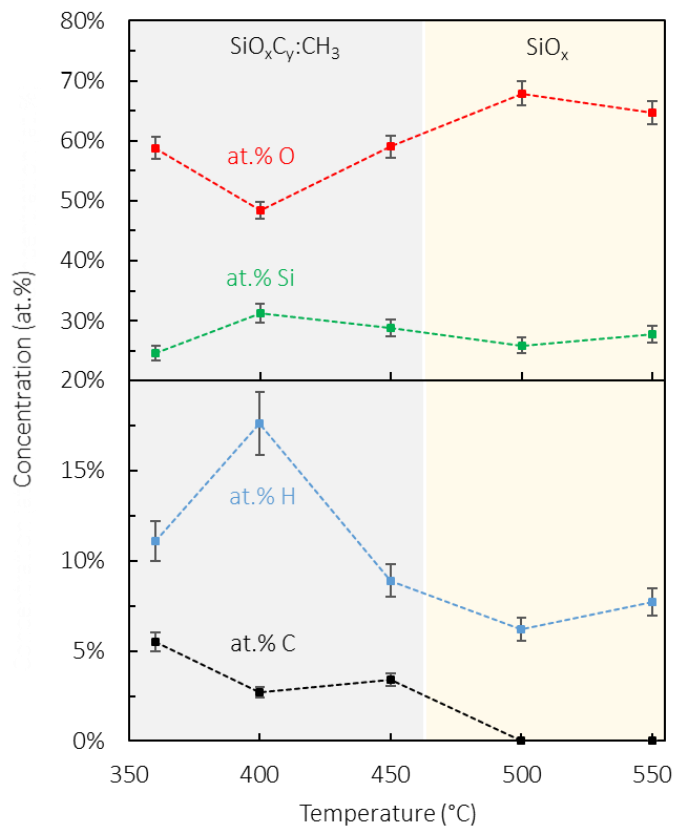
Figure 5. Evolution of HMDS-TEOS films composition as a function of SP temperature, obtained from the first spectral acquisition through IBA techniques. Grey and off-white areas signify \text{SiO}_x\text{C}_y\text{:CH}_3 and \text{SiO}_x material domains respectively.
