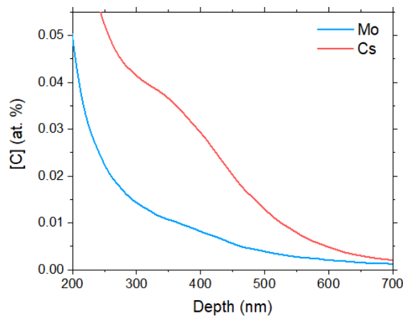
Figure 8: Concentration profiles of Cs and Mo in a \text{UO}_2 sample annealed at 1600^\circ\text{C} for 4 hours, in the 200-700 nm depth range.
