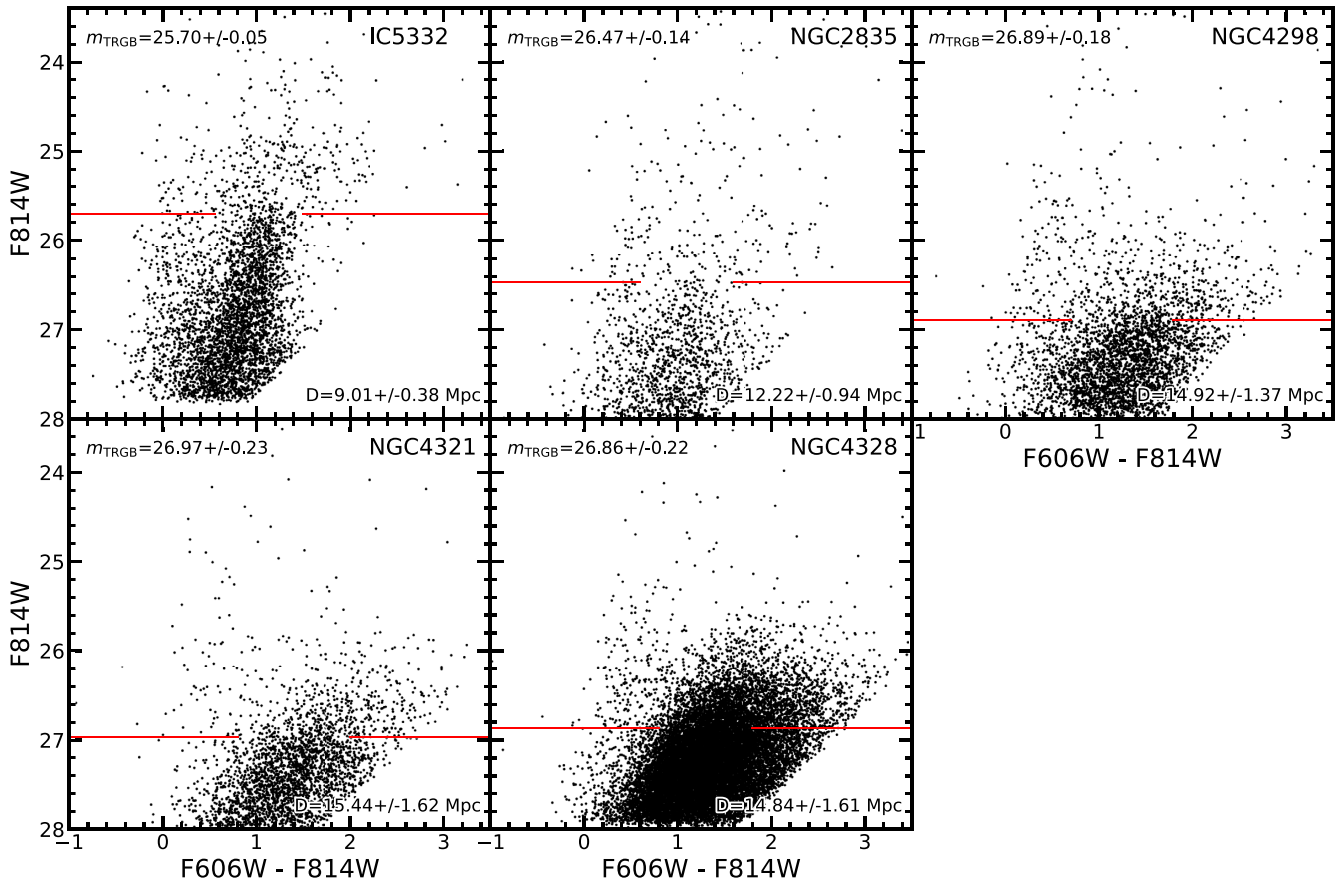
Figure 4. Same as Fig. 3, but for the five galaxies for which our TRGB measurements are the first.
