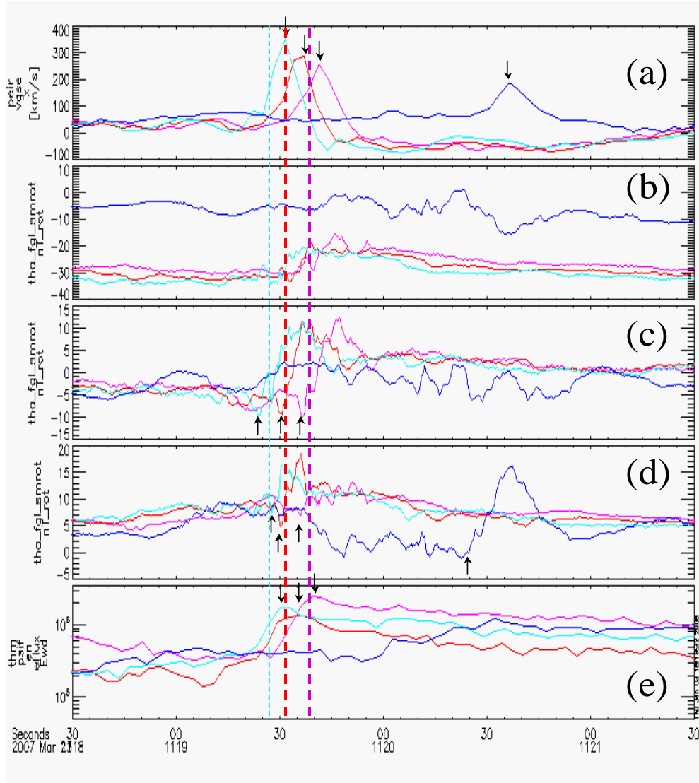
Figure 9. Timing of particles and fields signatures at the various spacecraft. THD, B, A and E are shown in Ciel, Red, Magenta and Blue, respectively, per the standard THEMIS color scheme, as in Figure 1 . The times are also tabulated in Table 2 . (a) X_{GSE} component of the flow velocity from the ESA instrument; (b), (c) and (d) X, Y, Z components of the magnetic field, in ‘rotated’ Solar Magnetospheric coordinates, where the X and Y axes have been rotated about Z_{SM} coordinate, such that X points towards Earth and Y is azimuthally westward; (e) the differential energy flux from the 40keV channel of the SST ions. TH-E was near the neutral sheet at the time, and saw no sharp signature in B_y and in energetic particles, but did experience the fast flow and the associated dipolarization.
