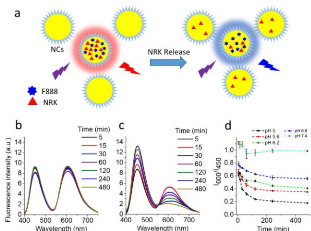
Fig. 1. (a) Schematic presentation of changes in FRET occurring during the cargo release. (b,c) Fluorescence spectra of Lipo-NRK NCs for different incubation time at pH 7.4 (b) and pH 5 (c) after dilution (1000-fold) in the presence of 20-fold excess of blank NCs. (d) Fluorescence intensity ratio of acceptor ( I_{600} ) to donor ( I_{450} ) over time at different pH. Excitation wavelength was 405 nm.
