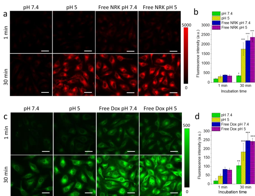
Fig. 4. pH-controlled release of cargos from NCs into cells, studied by fluorescence microscopy. (a) Fluorescence images of HeLa cells incubated for different time with Lipo-NRK NCs or free NRK at pH 5 and 7.4 (PBS). Excitation wavelength was 550 nm and the emission filter was 600 nm. (b) Mean fluorescence intensity measured in 13 cells from (a) excluding the nucleus area. (c) Fluorescence images of HeLa cells incubated for different time with Lipo-Dox NCs or free Dox at pH 5 and 7.4 (PBS). Excitation wavelength was 470 nm and the emission filter was 530 nm. Scale bars (a,c): 40 \mu m. (d) Mean fluorescence intensity measured in 13 cells from (c) excluding the nucleus area. Statistical analysis (vs. data at pH 7.4, 1 min): p < 0.5 (*), p < 0.1 (**), p < 0.01 (***)
