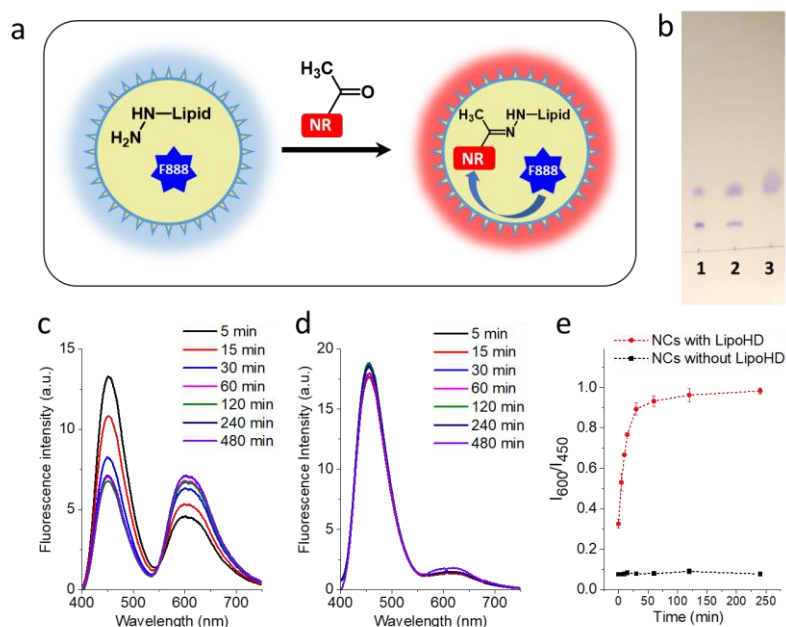
Fig. 2. (a) Scheme of in situ reaction of NRK and LipoHD monitored by FRET using F888 as energy donor. (b) TLC evidence of in situ formation of Lipo-NRK conjugate inside LipoHD NCs: (1) extracted reaction mixture of LipoHD NCs with NRK in DCM phase; (2) the same extracted mixture with pure Lipo-NRK; (3) pure Lipo-NRK. (c) Fluorescence spectra of the reaction mixture of LipoHD/F888 NCs with NRK at different reaction times after dilution (1000-fold) with 20-fold excess of blank NCs. Excitation wavelength is 405 nm. (d) The same experiments as (c) for NCs without LipoHD. (e) Fluorescence intensity ratio at fixed wavelengths (600 to 450 nm) for experiments (c) and (d). The in situ reaction was done at pH 4.
