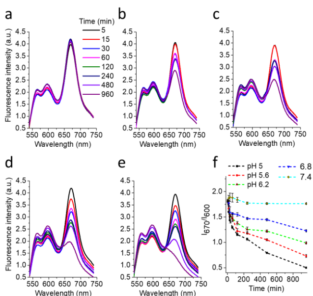
Fig. 3. Drug (Dox) release from NCs under pH control, studied by FRET from Dox to Cy5 dye (DiD). (a-e) Fluorescence spectra of Lipo-Dox FRET NCs (1000-fold dilution) in the presence of 20-fold excess of blank NCs at pH 7.4 (a), pH 6.8 (b), pH 6.2 (c), pH 5.6 (d) and pH 5 (e) over time. Excitation wavelength was 520 nm. (f) Fluorescence intensity ratio of acceptor to donor (670 to 600 nm) at different pH over time.
