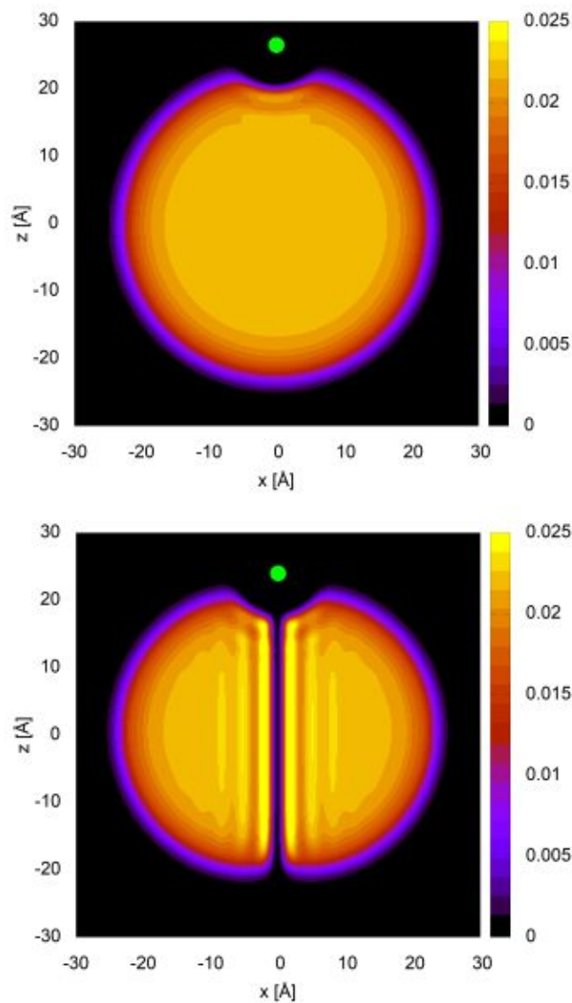
FIG. 1: 2D density in a plane of symmetry of a ^4\text{He}_{1000} droplet doped with a Cs atom (green dot). The color bar shows the He atom density in units of \text{\AA}^{-3} . Top, vortex-free droplet; bottom, vortex-hosting droplet.
