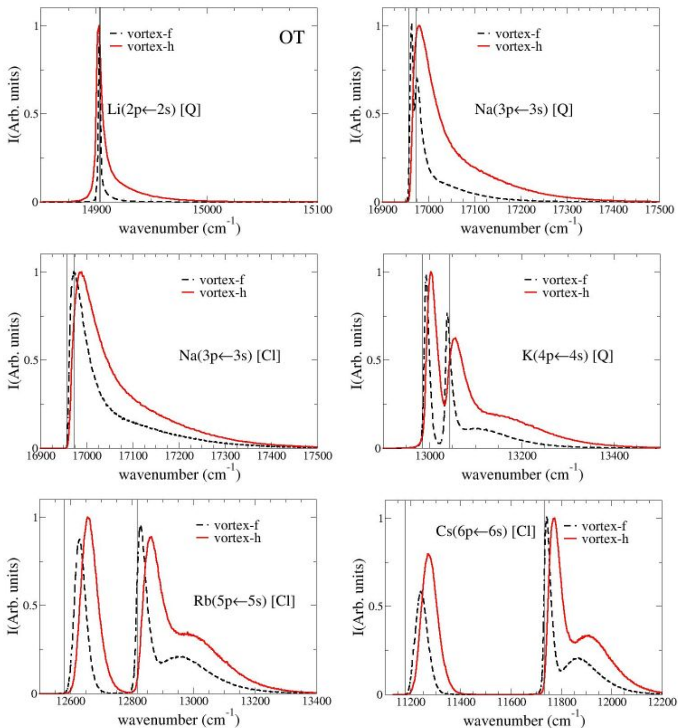
FIG. 2: np \leftarrow ns absorption spectrum for the alkali-doped ^4\text{He}_{1000} droplet obtained with the OT functional. Li, Na, and K atoms are treated quantum-mechanically ([Q]), whereas Rb, and Cs are treated classically ([Cl]). For the sake of comparison, the results for Na obtained with the classical description are also shown. Black dashed line: vortex-free (vortex-f) droplet; red solid line: vortex-hosting (vortex-h) droplet. Gas-phase atomic transitions are represented by thin vertical lines. Units are arbitrary for absorption intensity, and cm ^{-1} for excitation energy.
