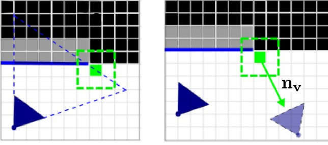
Fig. 3. [left] Two-dimensional example of ISE v (filled green square). Its 2D neighborhood is represented by a dashed green square. Unknown voxels are black, occupied are gray, and empty voxels are white. The reconstructed surface is depicted as a blue segment, and the sensor configuration and its frustum as dark blue triangles; [right] Direction from the contour, \mathbf{n}_v , and corresponding viewpoint configuration at distance \delta_{\text{pose}} from v (light blue triangle).
