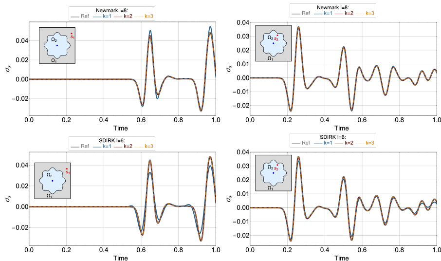
Figure 10: Flower-like test case. Comparison of the signal corresponding to \sigma_x at the sensors S_1 (left column) and S_2 (right column) for the Newmark scheme (upper row, time refinement level l = 8 ) and the SDIRK(3,4) scheme (bottom row, time refinement level l = 6 ). The results obtained with polynomial orders k \in \{1, 2, 3\} are compared to the reference solution.
