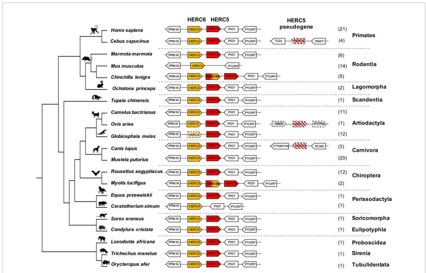
FIGURE 1 | Evolutionary dynamics of mammalian HERC5 and HERC6 gene loci. Representation of the HERC5 and HERC6 gene loci from mammalian genomes. Plain colored arrows represent intact HERC5 and HERC6 genes, striped colored arrows indicate HERC5 or HERC6 pseudogenes, and white arrows are adjacent syntenic genes. The newly identified chimeric HERC5/6 genes are bicolored. The numbers in brackets indicate the total number of genomes analyzed which contain the corresponding genomic organization in each mammalian order. In primates and carnivores, the HERC5 and HERC6 genes are well conserved. In the cetacean and rhinoceros' species, the HERC6 has been pseudogenized and lost, respectively, while rodent HERC5 has been lost in the Muridae and Cricetidae families. A duplicated HERC5/6 fused gene is independently fixed in several rodent species and in the Myotis genus in bats. Duplication followed by pseudogenization of HERC5 in primates, carnivores and artiodactyls is presented.
