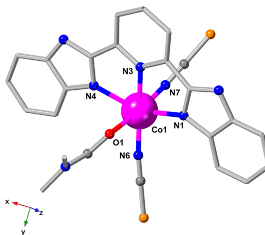
Figure 3. Perspective view of complex 2 . Hydrogen atoms and solvent molecules are omitted for clarity (Co, pink; C, gray; N, blue; O, red; S, orange).
