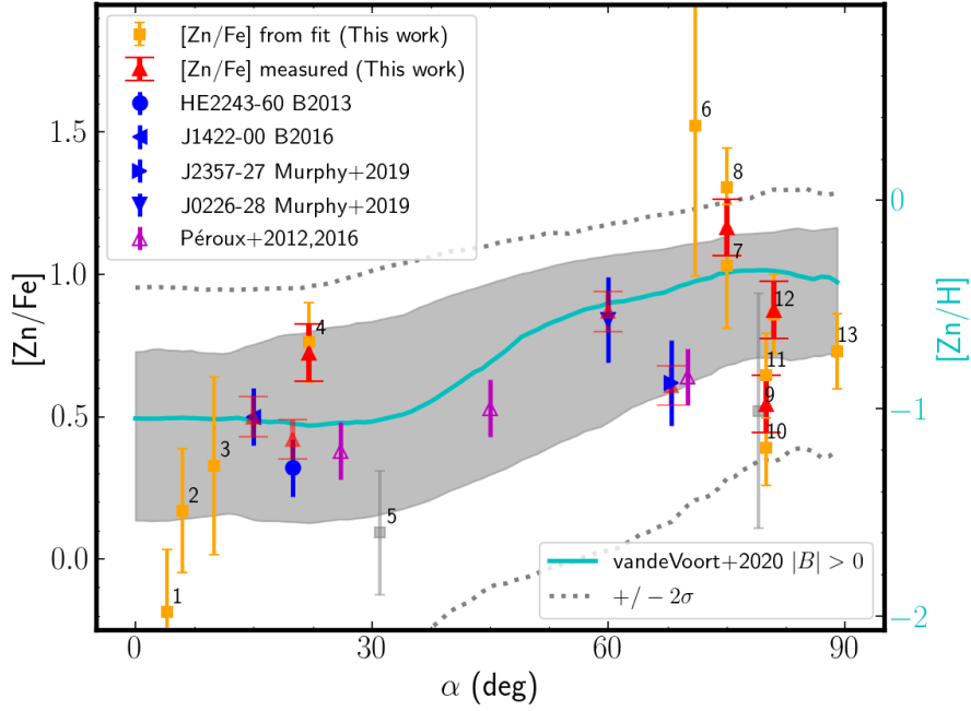
Figure 1. [\text{Zn}/\text{Fe}] depletion as a function of azimuthal angle \alpha from our galaxy-quasar pairs from MEGAFLOW using the depletion methodology of De Cia et al. (2016) described in section 3. The labeled IDs and their corresponding systems are listed in Table 1. For the right axis, the relation for a constant dust-to-gas ratio from De Cia et al. (2016) is used ( [\text{Zn}/\text{H}] = 1.37 \times [\text{Zn}/\text{Fe}] - 1.76 ). The cyan line represents the model from van de Voort et al. (2020) with non-zero magnetic field with their 1\sigma ( 2\sigma ) error as shaded (dotted lines), respectively. Individual literature data are shown from Péroux et al. (2012, 2016) (open triangles) and from Bouché et al. (2013, 2016); Murphy et al. (2019) (blue symbols, see also Table A2). The red symbols are direct measurements. The grey data points are possibly affected by saturation in Mg II.
