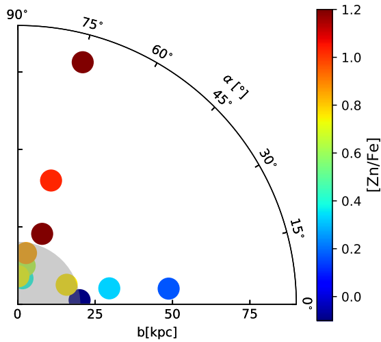
Figure 3. The position of the sightlines given as azimuthal angle \alpha at the distance (in kpc) and the obtained [\text{Zn}/\text{Fe}] color-coded. Blue data points represent lower metallicities ( [\text{Zn}/\text{Fe}] < 0.4 , mostly for lower angles, aligned to the major axis) red represents a higher metallicity ( [\text{Zn}/\text{Fe}] > 0.8 , mostly along the minor axis at higher azimuthal angles). The grey circle indicates the ISM region up to 20 kpc.
