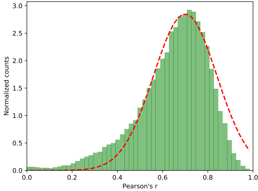
Figure 2. The distribution of the correlation coefficient for [\text{Zn}/\text{Fe}] against azimuthal angle for 50 000 bootstrap samples of the data plotted in Fig. 1. The Gaussian curve (red) correspond to r = 0.70 \pm 0.14 .
