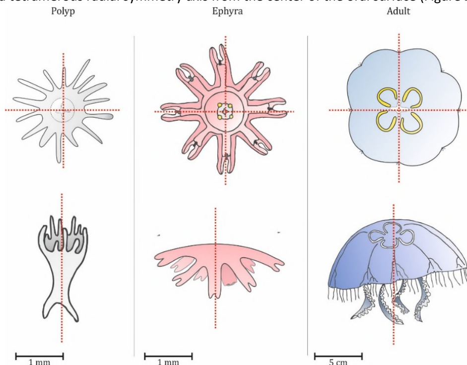
Figure 2. Symmetry at each stage of the Aurelia spp. jellyfish: tetramerous radial symmetry (oral face view) and vertical polar axis on polyp, ephyrae and medusae.
