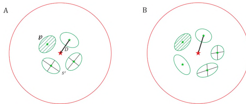
Figure 6. Conceptual scheme of the 3 different morphometric characteristics remarkable between the A: tetramerous jellyfish and B: the non-tetramerous jellyfish. \phi ratio rendering the relative size of the gonads; S^2 the individual variability of the gonad's eccentricity; D ratio rendering the relative distance of the gonad center to the umbrella center.
