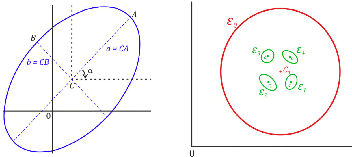
Figure 3. On the left: ellipse \mathcal{E} parameters; on the right: ellipses in a tetramerous jellyfish (with N = 4 gonads).
