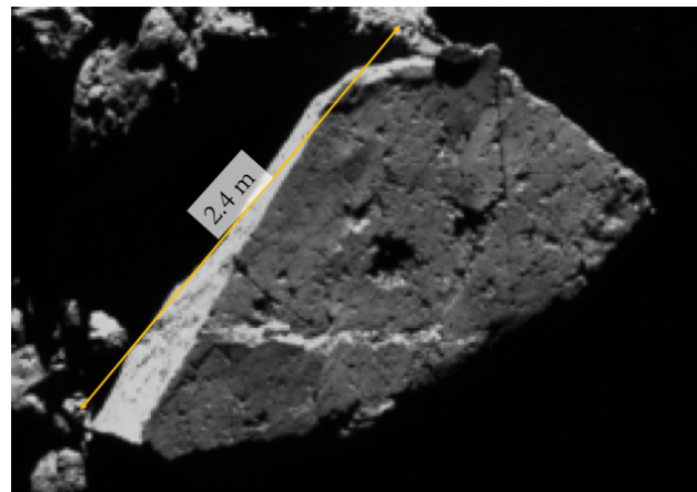
Fig. 1. OSIRIS-REx's Orbital B phase imaged Bennu's surface at pixel scales of ~1 cm/px, resolving centimeter-scale impact features, as evident on this boulder (image 20190703T044506S720_pol, taken July 3, 2019, by the OCAMS PolyCam imager).
