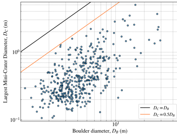
Fig. 2. A global search using the Bennu basemap [17] revealed 414 boulders with one or more impact features. For each boulder with impact features, its diameter ( D_B ), and its largest impact features ( D_C ). We find that a majority of boulders have impact features that have diameters below 50% of the host boulder's diameter (solid orange line).
