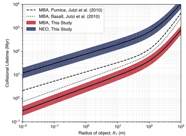
Fig. 3. C-type objects are weaker than porous pumice and non-porous basalt targets of the same size [6]. The red curve shows our derived collisional lifetime for C-type objects that are main belt asteroids (MBA) which have average impacts speeds of 5 km/s and a main-belt population and impact probability given by [3]. The blue curve shows the collisional lifetimes for C-type objects in near-Earth space based on impact speeds of 23 km/s and an NEO impactor population given by [18] and impact probability given by [3].
