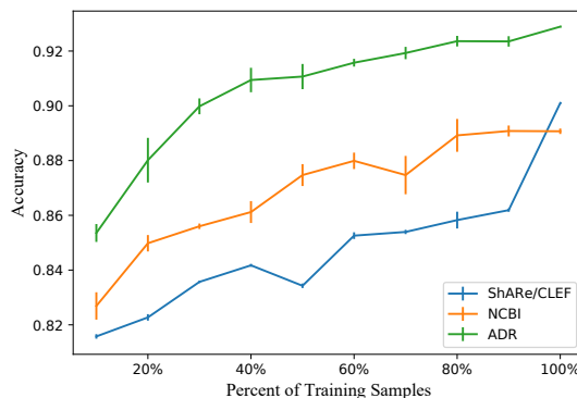
Figure 2: Model efficiency on a small amount of data.
