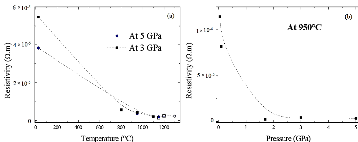
Figure 4. Resistivity of MgB 2 as a function of (a) temperature at 3 and 5 GPa and (b) pressure at 950 °C.
