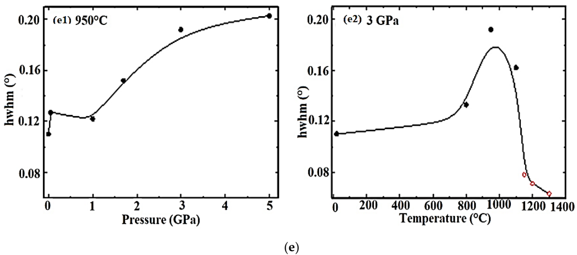
Figure 1. (a) Phase stability of MgB 2 with temperature at ambient pressure by in situ XRD. (b) Phase stability of MgB 2 with temperature at 100 MPa and decomposition of MgB 2 at 1250 °C. (c) Phase stability of MgB 2 with temperature at (c1) 3 GPa and (c2) 5 GPa. (d) Phase stability of MgB 2 with pressure at 950 °C (e) Evolution of peak (101) width by XRD on MgB 2 with (e1) Pressure at 950 °C and (e2) Temperature at 3 GPa.
