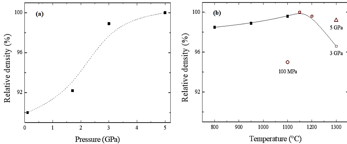
Figure 2. Density of MgB 2 with (a) Pressure at 950 °C and (b) Temperature at 3 GPa (red hollow symbols stand for decomposed samples).
