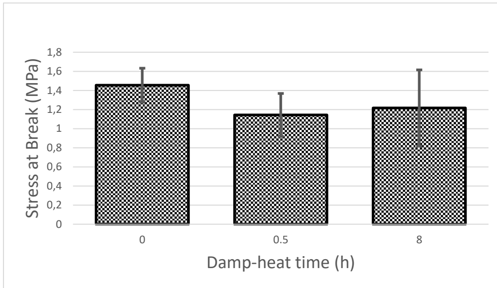
Figure 4. Evolution of the stress at break for fresh and degraded devices upon damp heat with time.
