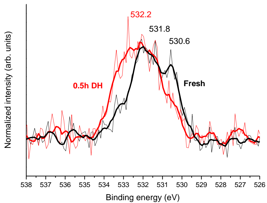
Figure S1. Normalized XPS spectra in the O1s region of the fresh and 0.5h DH delaminated samples.
