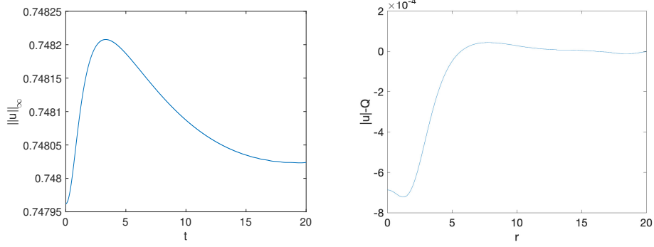
FIGURE 8. The 2D solution u to (1.1) for initial data (4.2) with \omega = 0.1 and \lambda = 0.99 . On the left the L^\infty -norm as a function of time. On the right the difference between |u| and Q_{\omega=0.1} at the final time t_f = 20 .
