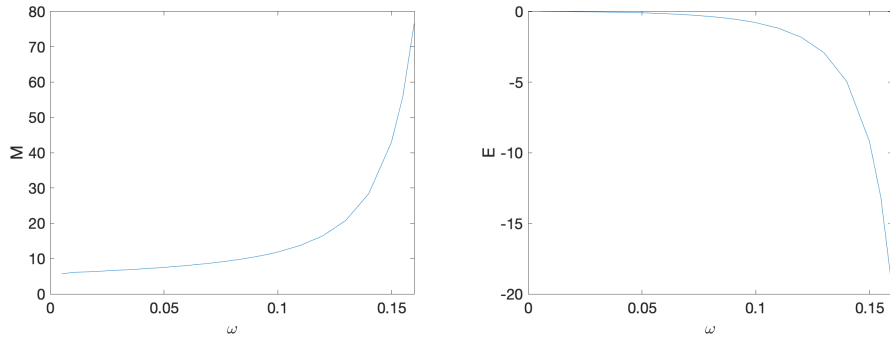
FIGURE 3. M(Q_\omega) and E(Q_\omega) as a functions of \omega in dimension d = 2 .
