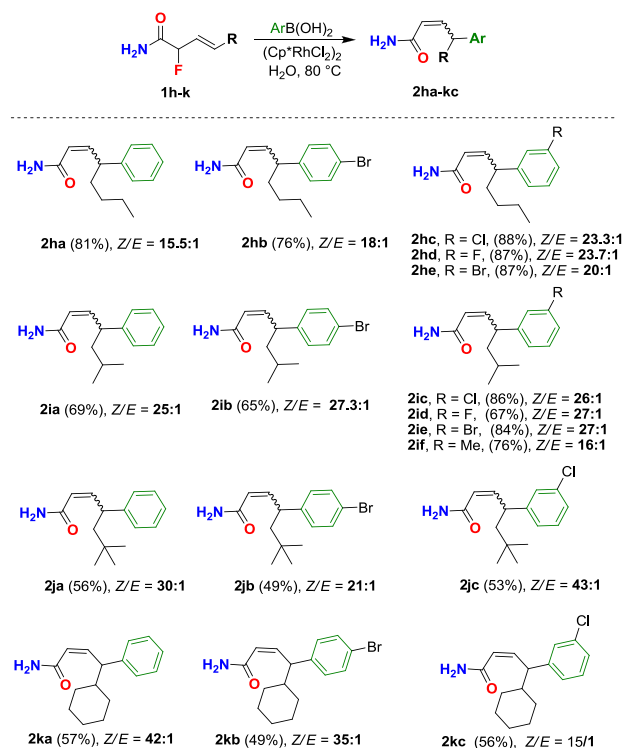
Scheme 3. Investigation of the primary amide substrates scope a,b,c
