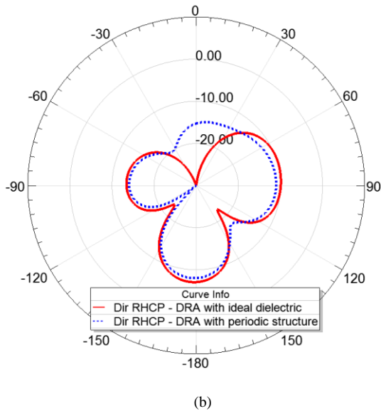
Fig. 8. Simulated (a) left-hand and (b) right-hand CP directivity (dBi) of the DRA using an ideal anisotropic dielectric and periodic structure at f_0=2.45 GHz and \phi=0^\circ .
