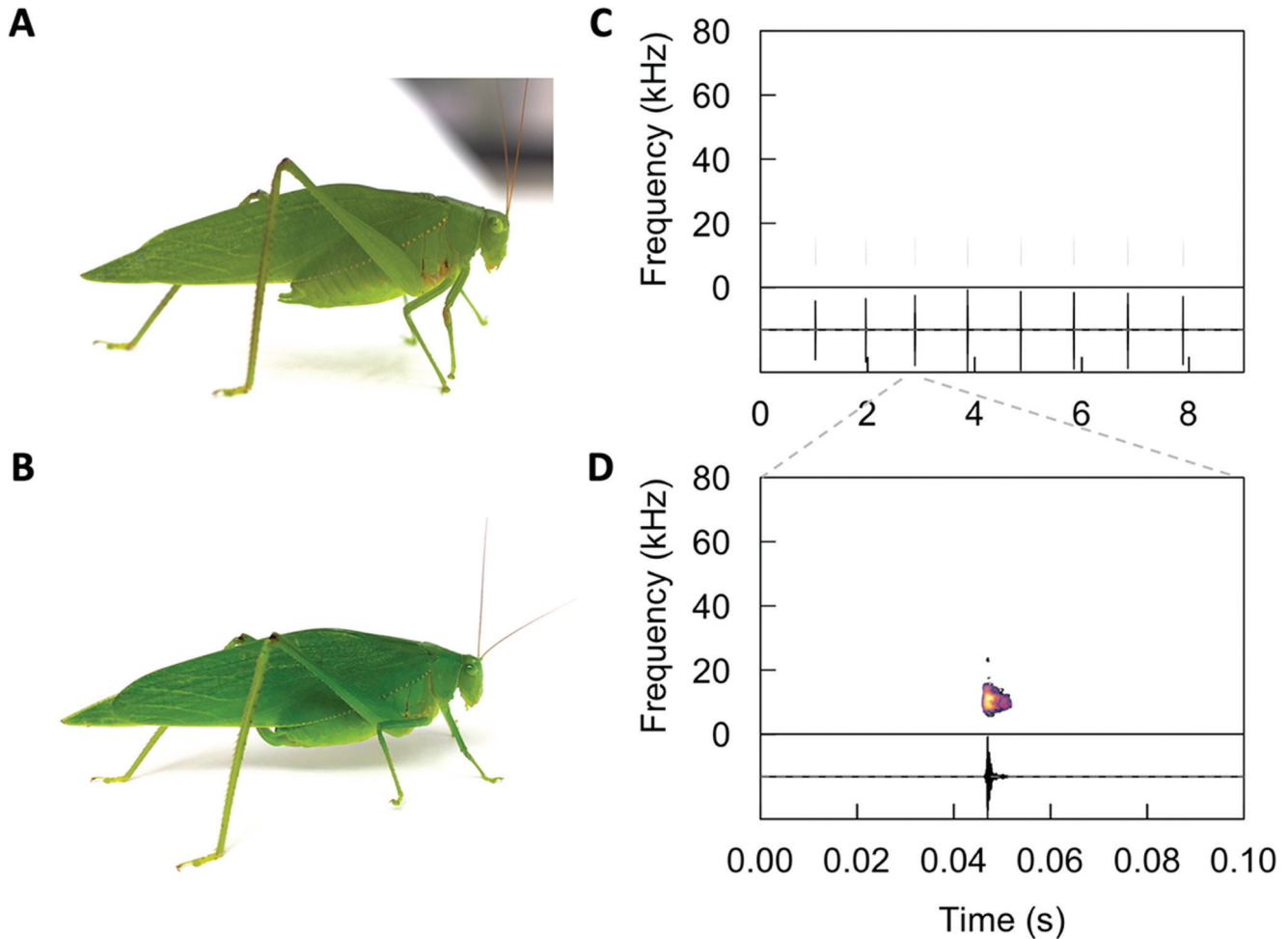
Fig. 32. Photographs and calling song spectrograms of Microcentrum "polka". A. Male (photo credit: C. Kernan); B. Female (photo credit: L. Symes); C. and D. Spectrogram (top panel) and oscillogram (bottom panel) of one call (C) and one pulse from the same call (D).
