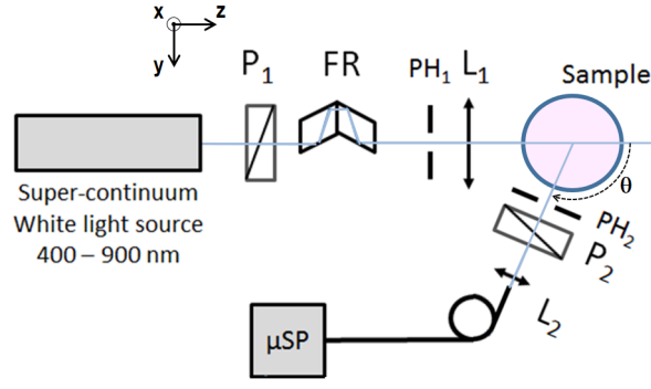
Fig. 5 Static light scattering setup. P_1 and P_2 are broadband polarizers, FR is a Fresnel rhomb tandem, L_1 and L_2 are lenses and PH_1 and PH_2 are pinholes. \mu\text{SP} is a spectrophotometer. \theta is the scattering angle and varies from 20 to 140°.
