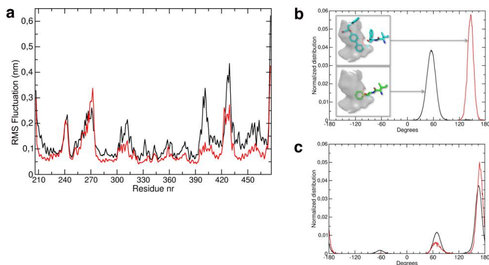
Figure 8. Molecular dynamics simulation.
