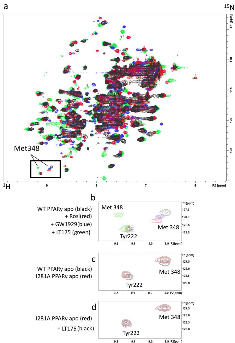
Figure 5. ^1\text{H} - ^{15}\text{N} HSQC NMR spectra.
