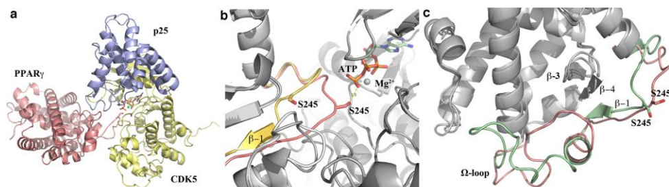
Figure 1. Docking study on the interaction between the CDK5/p25 complex and PPAR \gamma .
