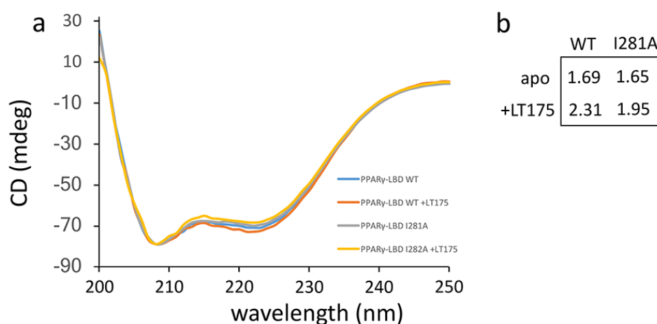
Figure 6. CD spectra.
