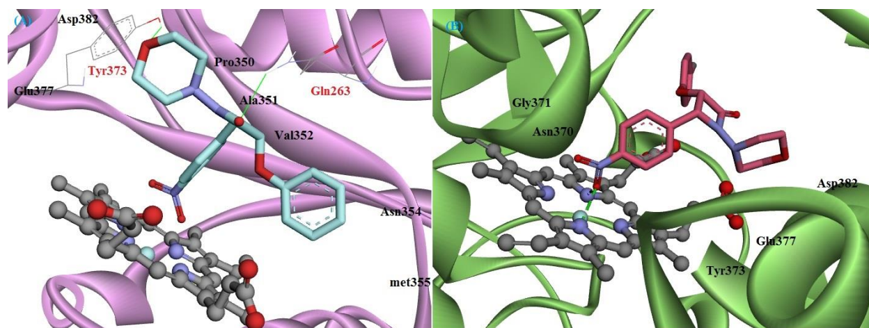
Fig. 4. Computational binding modes of compound 3a (A) and 3b (B) in the active site of human inducible nitric oxide synthase.
