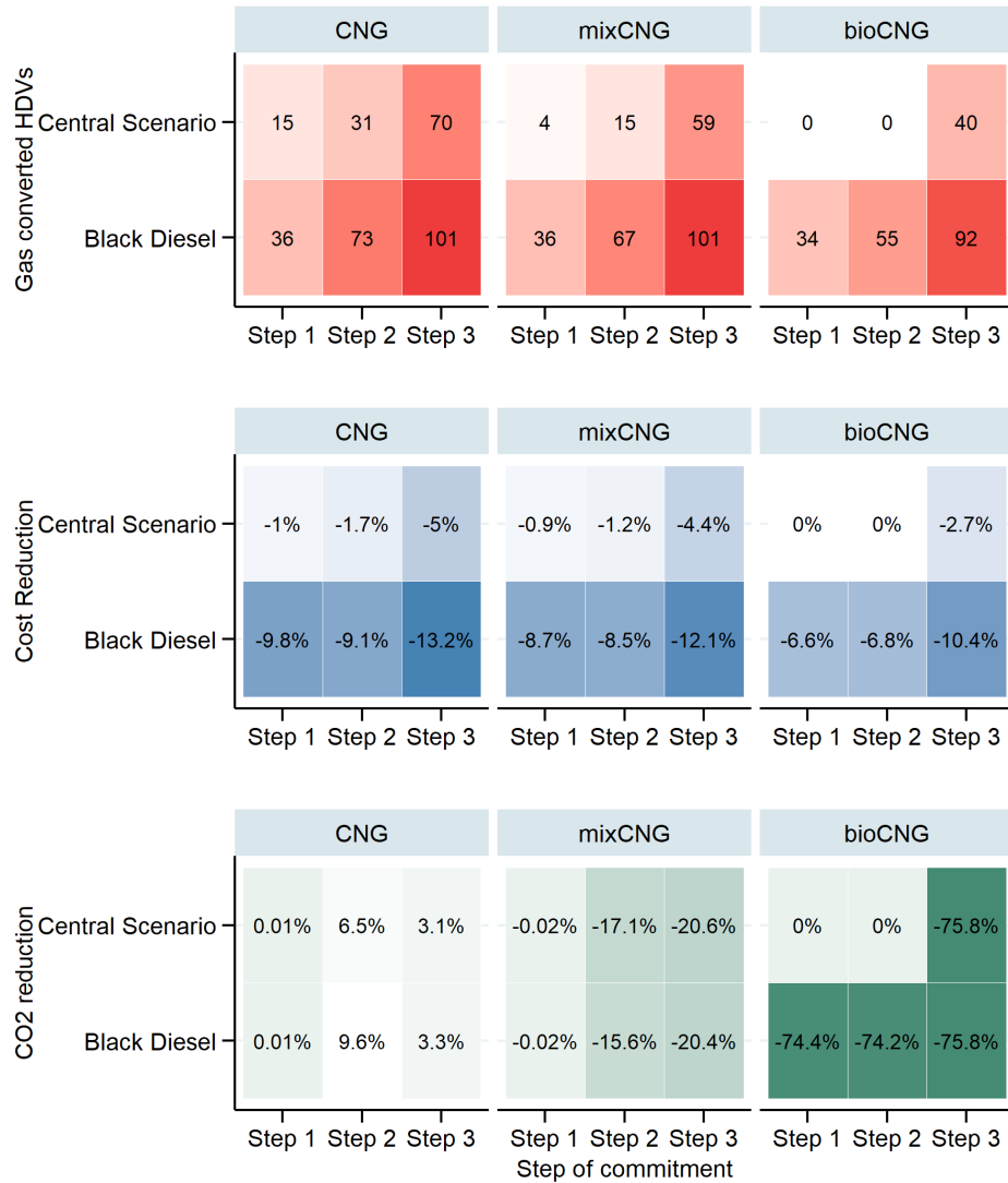
FIGURE 2: Cost and emissions reductions for each scenario
