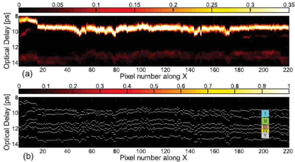
Figure 2. (a) THz B-scan based on the raw measured data and (b) Binary THz B-scan based on the deconvolved data for a typical cross-section, in which a valid peak is assigned value '1' and the other positions '0' regardless of the sign or height of the peak. I: varnish; II: pictorial layer; III: underpainting; IV: imprimatura; V: ground layer.
