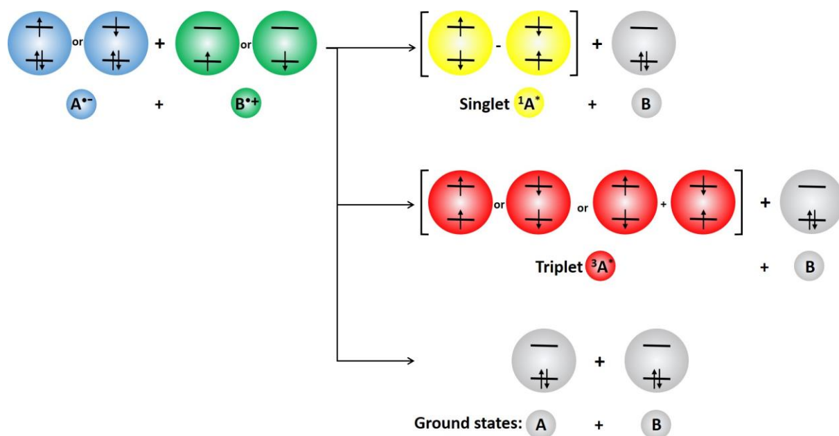
Figure 6. a) Schematic representation of the bimolecular electron-transfer reaction between the radical species A^{\bullet} and B^{\bullet} . For energy-sufficient reaction, spin statistics dictate the singlet/triplet ratio with the formation of 25% singlet states ^1A^* (spins antiparallel with zero resultant spin angular momentum) and 75% triplet states ^3A^* (spins parallel, with three resulting nonzero spin angular momentum vectors).
