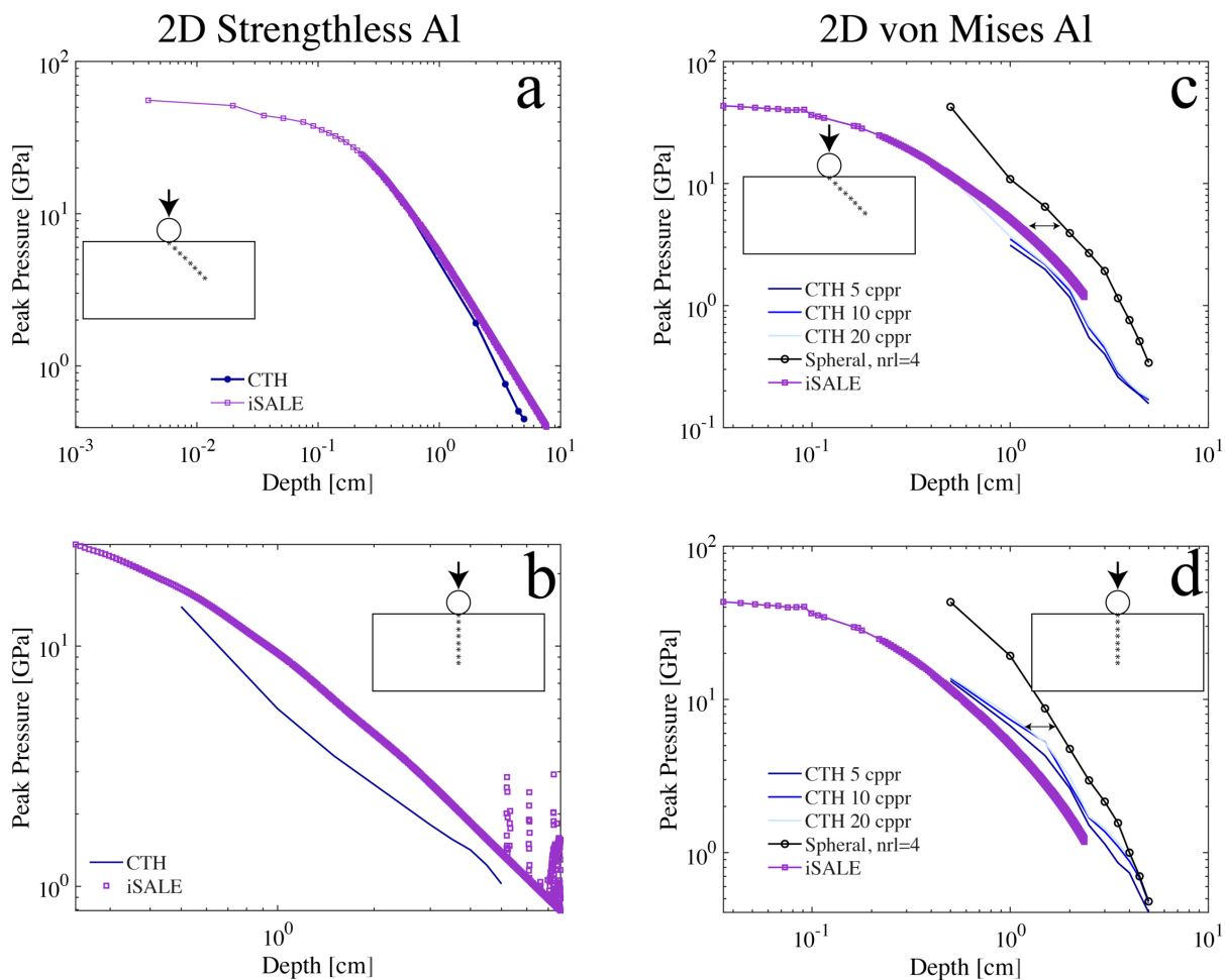
594 595 596 Figure 5. Pressure as a function of depth for impacts into strengthless aluminum (left) and 597 aluminum with a constant strength (right) for simulations using CTH, iSALE, and Spheral. The 598 offset in the Spheral simulation is likely due to difficulty of defining stationary Eulerian tracer 599 points in a meshless code, which is a relatively new capability in Spheral. 600
