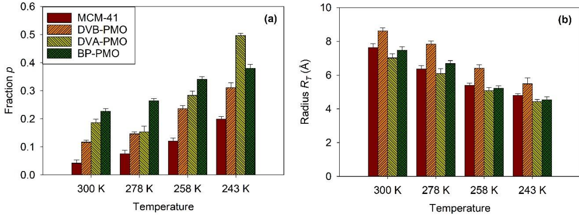
FIG. 6. Variation with the temperature and the confining matrix of the parameters obtained from the fit of the EISF of the translational diffusion (from IN5B measurements). (a) Fraction p of dynamically frozen water molecules. (b) Radius R_T of the sphere confining the translational diffusion.
