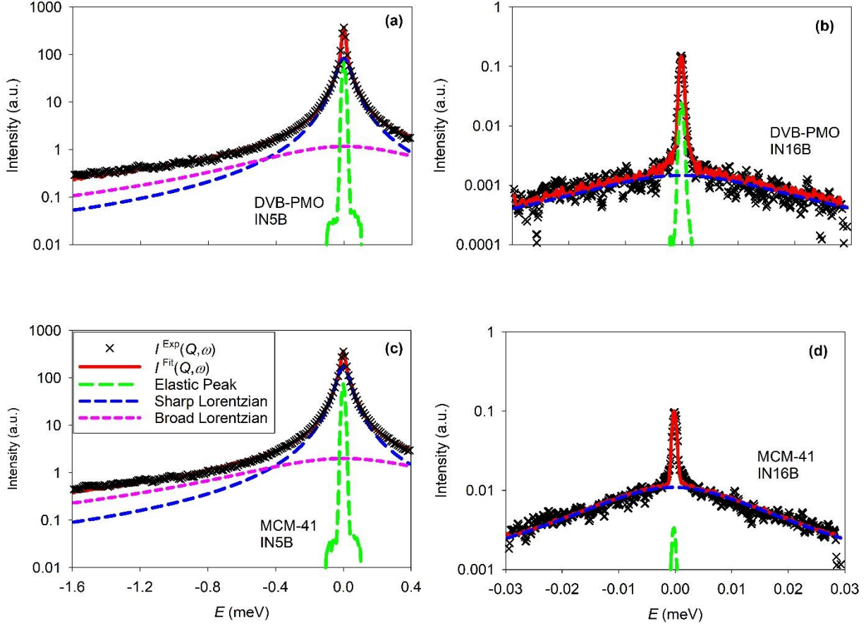
FIG. 3. QENS spectra (cross symbols) and fitted functions (lines) at the temperature T = 278 K of water confined in DVB-PMO (upper panels a, b) and in MCM-41 (lower panels c, d). QENS spectra measured on IN5B at Q = 0.8 \text{ \AA}^{-1} (left panels a, c) and on IN16B at Q = 0.85 \text{ \AA}^{-1} (right panels b, d).
