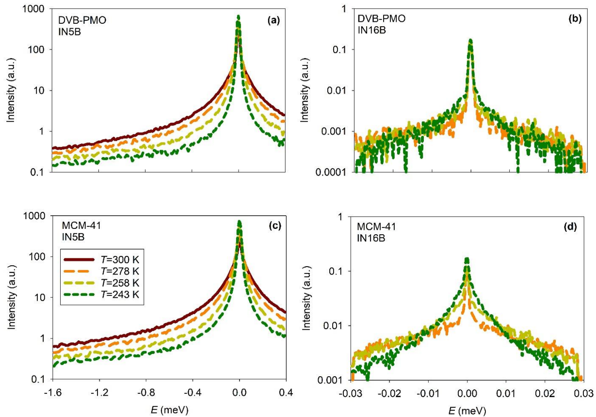
FIG. 1. Temperature dependence of the scattering intensity of water confined in DVB-PMO (upper panels a, b) and in MCM-41 (lower panels c, d). QENS spectra measured on IN5B at Q = 0.8 \text{ \AA}^{-1} (left panels a, c) and on IN16B at Q = 0.85 \text{ \AA}^{-1} (right panels b, d).
