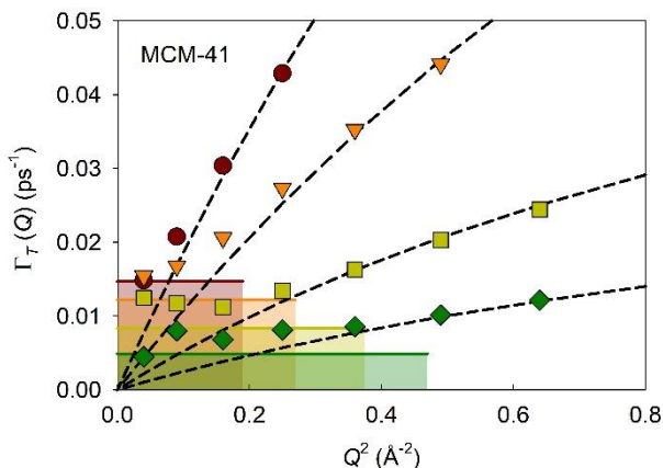
FIG. 8. Enlarged view of the half width at half-maximum \Gamma_T in the region of small Q s for water confined in MCM-41 at the same four temperatures (filled symbols) as shown in Fig. 7(a). Fit using the jump diffusion model (thin dashed lines). The level of the low Q limits predicted by the model of diffusion inside a sphere are illustrated by shaded areas. 54
