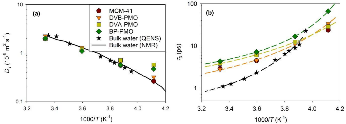
FIG. 9. (a) Translational diffusion coefficient D_T and (b) residence time \tau_0 of water evaluated from the fit of IN5B spectra with a jump-diffusion model for water confined in MCM-41 and three PMOs as a function of the inverse temperature. In panel a, the QENS data of bulk water are from Teixeira et al. 47 (stars) and the NMR diffusion coefficient from Price et al. 59 (solid line). VTF fits of the residence time (dashed line in panel b).
