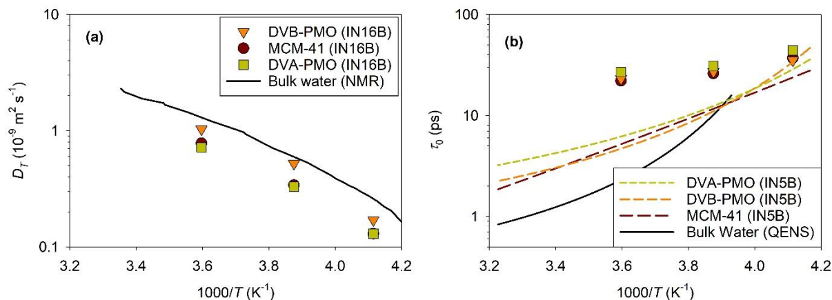
FIG. 11. (a) Translational diffusion coefficient D_T and (b) residence time \tau_0 of water evaluated from the fit of IN16B spectra with a jump-diffusion model for water confined in MCM-41 and two PMOs as a function of the inverse temperature (symbols). In panel a, the NMR diffusion coefficient of bulk water from Price et al. 59 (solid line). In panel b, the residence time of water confined in the same matrices fitted from IN5B spectra (dashed line) and the residence time of bulk water from Teixeira et al. 47 (solid line)
