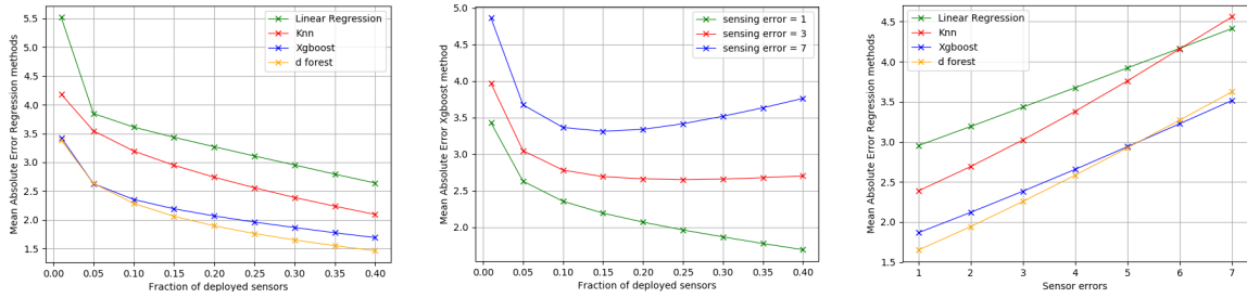
Fig. 3 (a) MAE Vs percentage of deployed sensors, \sigma_m = 1 \mu\text{g}/\text{m}^3 ; (b) MAE of Xgboost method Vs percentage of deployed sensors, s \in [1, 3, 7] ; (c) MAE Vs Standard error deviation, Fraction of deployed sensors = 0.3
