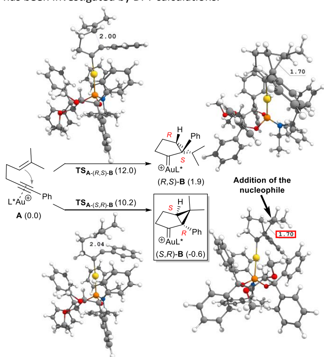
Scheme 4. Free energies ( \Delta G_{253} , kcal/mol) and selected distances ( \text{\AA} ) of the computed species.
