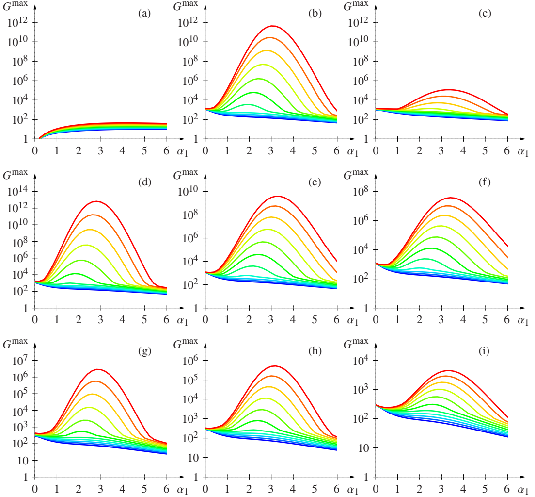
Figure 16: Maximum energy growth G^{\max} for pulsating pipe flows, over 0 < \alpha_1 < 6 at \tilde{Q} = 0.0, 0.1, 0.2, \dots, 1.0 . Here (a–f) \text{Re} = 4000 and (g–i) \text{Re} = 2000 ; (a–c,h) \text{Wo} = 10 , (d,g) \text{Wo} = 8 , (e) \text{Wo} = 12 and (f,i) \text{Wo} = 14 ; (a) \alpha_2 = 0 , (b,d–i) \alpha_2 = 1 and (c) \alpha_2 = 2 .
