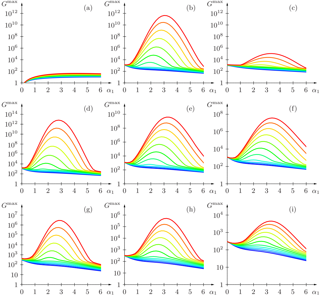
FIGURE 16. Maximum energy growth G^{\max} for pulsating pipe flows, over 0 < \alpha_1 < 6 at \tilde{Q} = 0.0, 0.1, 0.2, \dots, 1.0 . (a–f) \text{Re} = 4000 , and (g–i) \text{Re} = 2000 . (a–c, h) \text{Wo} = 10 . (d, g) \text{Wo} = 8 , (e) \text{Wo} = 12 , (f, i) \text{Wo} = 14 . (a) \alpha_2 = 0 . (b, d–i) \alpha_2 = 1 . (c) \alpha_2 = 2 .
