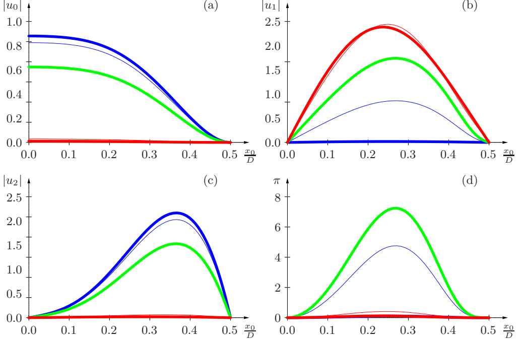
FIGURE 10. Evolution of spatial structure of maximally amplified streaks for \text{Re} = 4000 , \text{Wo} = 10 and \tilde{Q} = 0.1 . Spatial profiles of flow fields (normalised to unit total energy) over half channel 0 \leq x_0 \leq D/2 at different snapshots: t_i = 0.166T optimal initial perturbation (thick blue lines), t = 0.169T (thin blue lines), t_\star = 0.175T at maximum growth rate (thick green lines), t = 0.500T (thin red lines), t_f = 1.389T optimal response (thick red lines). Envelope of wall-normal |u_0(x_0, t)| (a), streamwise |u_1(x_0, t)| (b) and spanwise |u_2(x_0, t)| (c) velocity perturbation. Energy production \pi(x_0, t) (d) terms.
