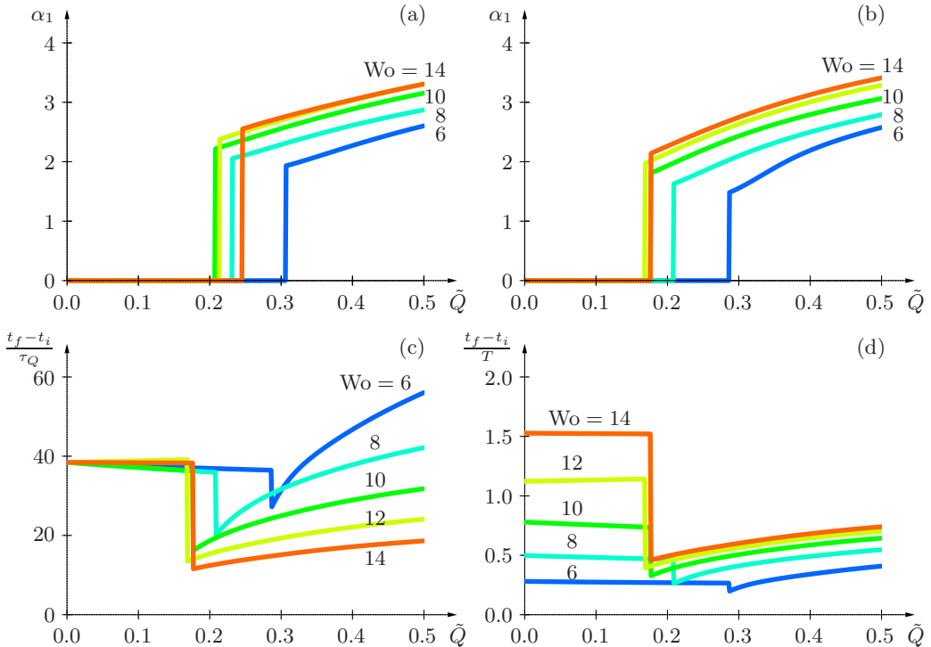
FIGURE 19. Characterization of the maximally amplified optimal perturbations as the pulsation amplitude \tilde{Q} is increased for Wo = 6, 8, 10, 12, 14 . Streamwise wavenumber \alpha_1 at (a) \text{Re} = 2000 and (b) \text{Re} = 4000 . Duration of transient growth t_f - t_i at \text{Re} = 4000 (c) measured in mean-flow advection units \tau_Q and (d) in pulsation periods T .
