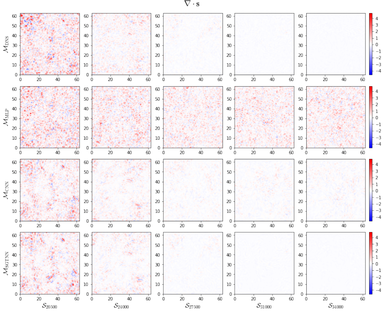
FIG. 9. Data slices of the predicted SGS terms from NN models in scalar decay regime. It is particularly visible that \mathcal{M}_{MLP} and \mathcal{M}_{CNN} are still predicting a non-null SGS term when the scalar is completely mixed.
