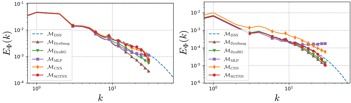
FIG. 17. Energy spectrum of simulation in full decay regime starting from testing data at t = 8 (left) and t = 30 (right).
