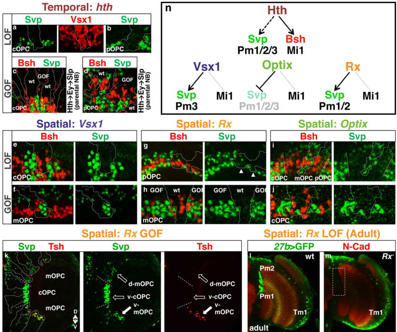
Figure 3. Temporal and spatial inputs are required for neuronal specification in the medulla a. In hth mutant MARCM clone, Svp expression (green) is lost but Vsx1 (red) is unaffected in the cOPC. b. Svp expression (green) is lost in the pOPC in hth mutant MARCM clone. c and d. Bsh (red) is ectopically expressed in the progeny of older neuroblasts in hth gain-of-function (GOF) clones in the cOPC (c) or in the pOPC (d). Svp expression (green) is unaffected in both case (c and d). e–j. Bsh (red) and Svp (green) expression in different LOF and GOF. e. Vsx1 RNAi loss-of-function (LOF) clone in the cOPC. f. Vsx1 GOF clone in the mOPC. g. Rx LOF mutant MARCM clone in the pOPC. h. Rx GOF clones in the mOPC. i. Optix LOF mutant MARCM clone in the mOPC. j. Optix GOF clone in the cOPC.
