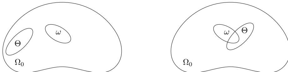
Figure 1: The two main situations investigated: (left) the intersection set of \omega and \Theta is empty; (right) the intersection set of \omega and \Theta is nonempty.
