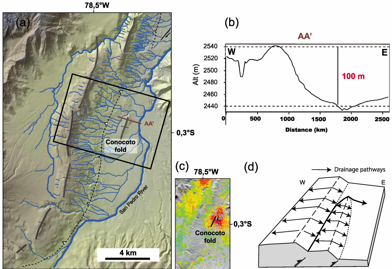
Figure 9. (a) Drainage map on the Inter-Andean valley, east of the Quito Basin and neotectonic interpretation (modified from Alvarado 2012). (a) Blue curves are rivers; thick black lines are the top fold locations and the dashed black line with triangles is the surface location of the main thrust fault. Note the deflection of the drainage system to the north around the Conocoto fold. Black rectangle is the location of the inset (b) and (d). (b) Topographic profile across the Conocoto fold. (c) Same area as in (a) with the LOS surface velocity from Fig. 3(a) compared with the location of the Conocoto fold. (d) Propagation model of thrust (inspired from Jackson et al. 1996).
