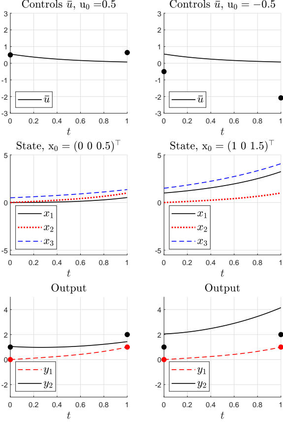
Fig. 3. Time trajectories of the controls transferring y_0 = (0 \ 1)^T on y_1 = (1 \ 2)^T in time T = 1 for the system given in Example 6.2. The control \bar{u} is computed for two different values of (x_0^T, u_0^T)^T in \Gamma_{y_0} .
