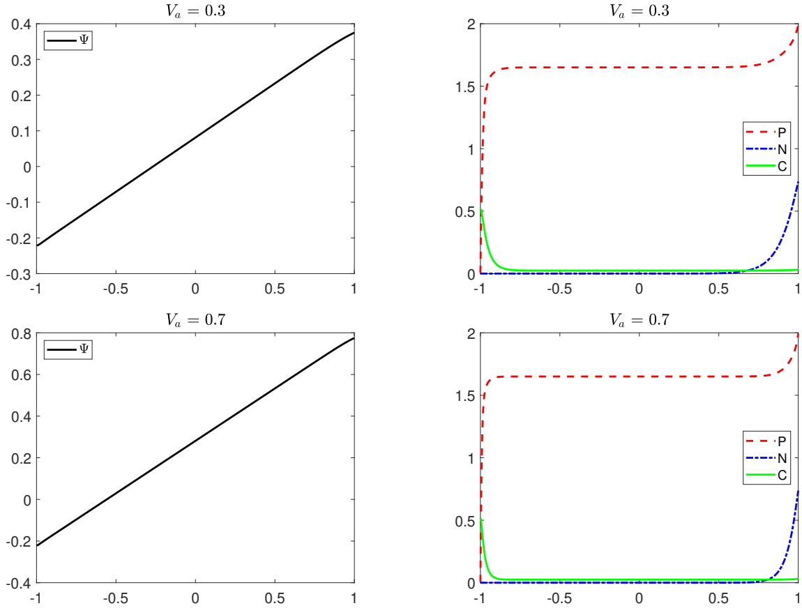
FIGURE 3. A pseudo-stationary steady state for pH = 7 and V_a = 0.3 Volts (top) and V_a = 0.7 Volts (bottom).
