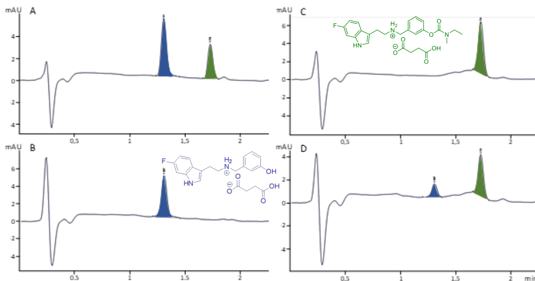
Figure 5. Decarbamylation of 18 by eqBuChE ; (A): 18 (5 μM) and 17 (5 μM) calibration range; (B): 18 (5 μM) without eqBuChE (negative control); (C): 17 (5 μM) without eqBuChE (negative control); (D): 18 (5 μM) in the presence of 250 U/mL eqBuChE ; 25°C, 18 h, λ = 280 nm.
