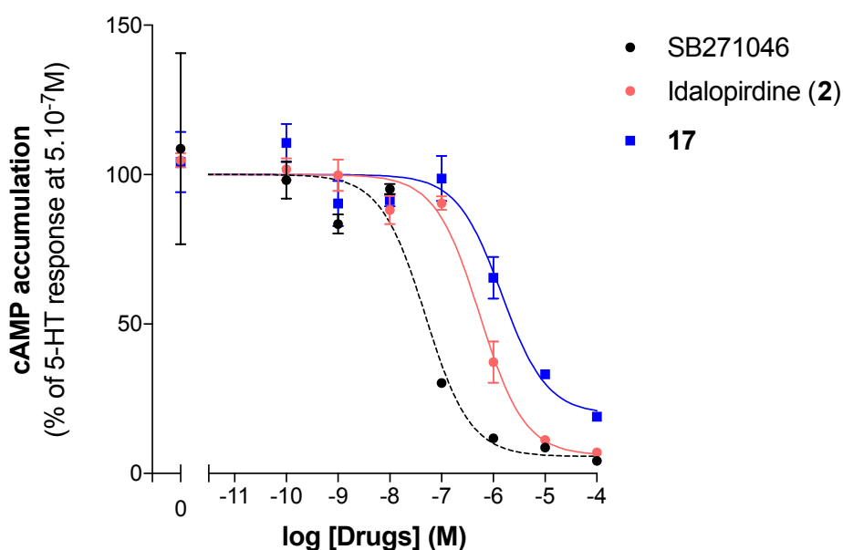
Figure 3. Pharmacological profiles of idalopirdine ( 2 ) and compound 17 . Representative experiment illustrating antagonist activities towards h5 -HT 6 receptors.
