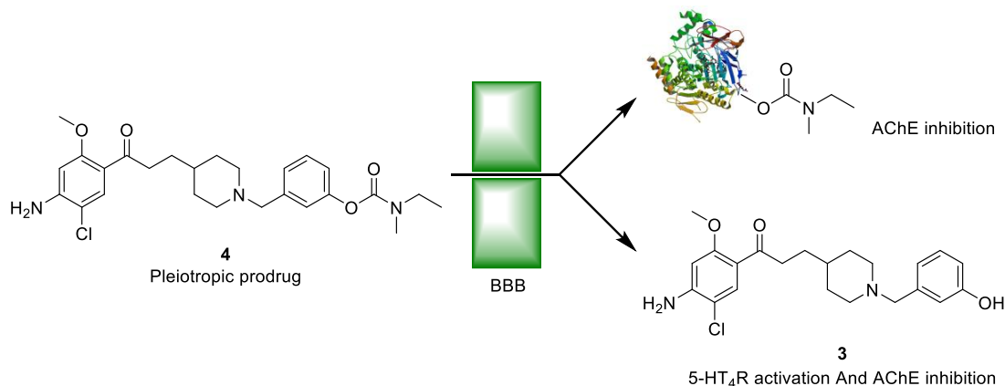
Figure 2. Illustration of mechanism of action of the pleiotropic prodrug related to donecopride [31].
