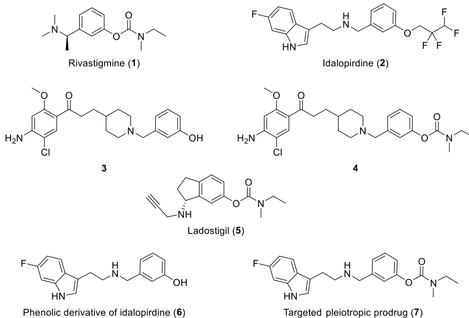
Figure 1. Structure of rivastigmine ( 1 ), idalopirdine ( 2 ), 3 , 4 , ladostigil ( 5 ), phenolic derivative of idalopirdine ( 6 ) and targeted pleiotropic prodrug ( 7 ).
