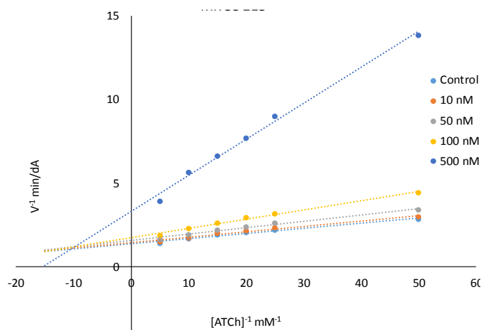
Figure 4. Lineweaver-Burk plots of inhibition kinetics show that carbamate 18 acts as a mixed-type eq BuChE inhibitor.
