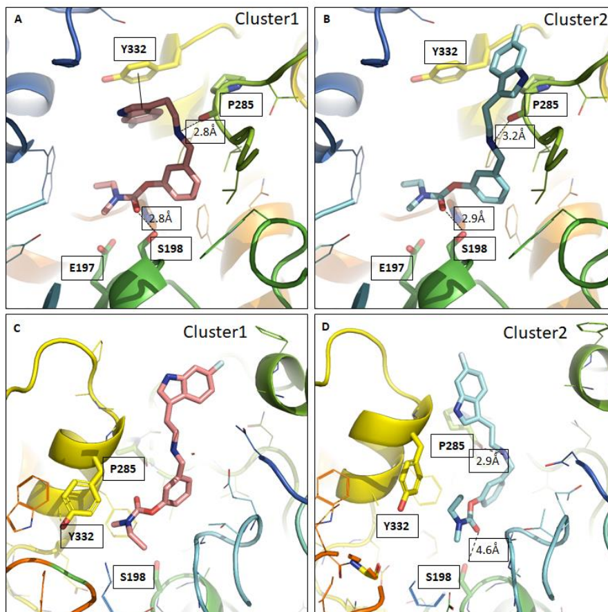
Figure 6. The two representative positions of compound 18 in h BuChE binding sites generated from the docking studies, cluster 1 ( A ) and cluster 2 ( B ) and the representative structure from their molecular dynamics simulations, cluster 1 ( C ) and cluster 2 ( D ). The compound and the selected side chains of the binding site residues are in stick and the protein in ribbon representation. This figure was made with PYMOL (DeLano Scientific, 2002, San Carlo, USA).
