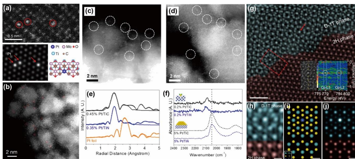
Figure 3 | Metal (hydr)oxides / nitrides / carbides / sulfide as supports for SACs. (a) HAADF-STEM image of \text{Mo}_2\text{TiC}_2\text{Tx} -Pt SACs and its corresponding simulated image. Reproduced from Ref. [39] with permission from Nature Publishing Group. (b) HAADF-STEM image of Pt/ \alpha -MoC with the single Pt atoms circled. Reproduced from Ref. [42] with permission from Nature Publishing Group. (c-f) Single-atom Pt loaded on TiC and TiN characterized by the HAADF-STEM, Pt L3 edge k^3 -weighted FT-EXAFS spectra and diffuse reflectance FT-IR spectra. Reproduced from Ref. [43] with permission from the American Chemical Society. (g-j) HAADF-STEM characterization of SA Co-D 1T \text{MoS}_2 , which shows the obvious junction between SA Co-D 1T \text{MoS}_2 and pristine 2H \text{MoS}_2 . Reproduced from Ref. [48] with permission from Nature Publishing Group.
