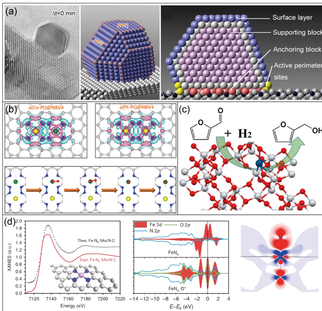
Figure 12 | Identification of the active sites for the SACs. (a) TEM schematic depicting a typical gold nanoparticle atomic scheme of a gold nanoparticle anchoring onto a CeO 2 nanorod, which illustrates the functions of different domains. Reproduced from Ref. [140] with permission from the American Chemical Society. (b) Top view of the charge densities of SA Co on N-doped carbon and SA Pt on the same support. Pink and aqua represent the electron accumulation and depletion areas, respectively. The ORR reaction pathway is illustrated below. Reproduced from Ref. [147] with permission from the American Chemical Society. (c) Experimental results show that the single-atomic-site Ir catalyst supported by the defective metastable phase of titanium dioxide exhibits excellent catalytic performance for the hydrogenation of furfural to furfuryl alcohol. Reproduced from Ref. [149] with permission from the American Chemical Society. (d) XANES spectra, partial density of states (PDOS) and charge density differences analyses of Fe-N 4 SACs. Reproduced from Ref. [150] with permission from the American Chemical Society.
